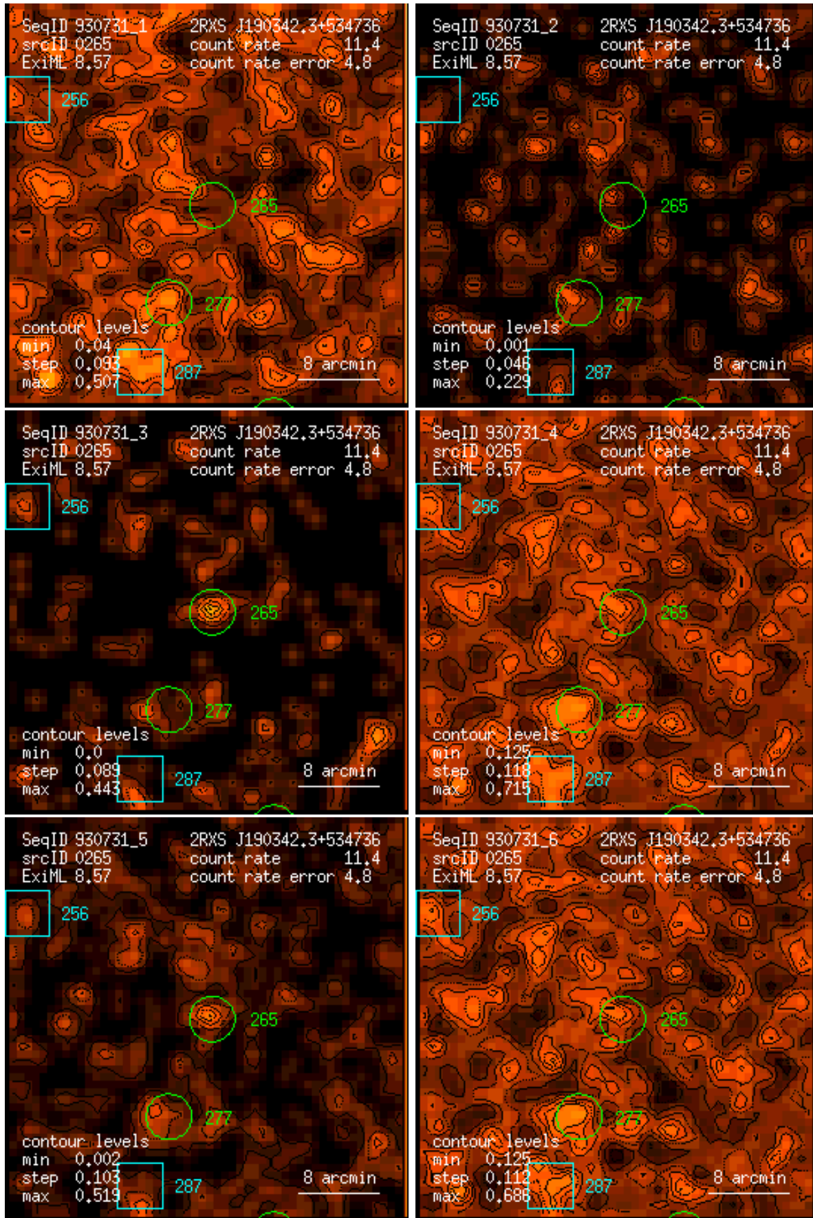
Figure 265: RASS 930731: detection 0265: band rate images, Gaussian filter: (1) PSPC channels 11 – 41, (2) 52 – 90, (3) 91 – 201, (4) 11 – 235, (5) 52 – 201, (6) 11 – 201. Broad band rates in counts/ks. Band rate contour levels in counts/ks/arcmin 2 .
