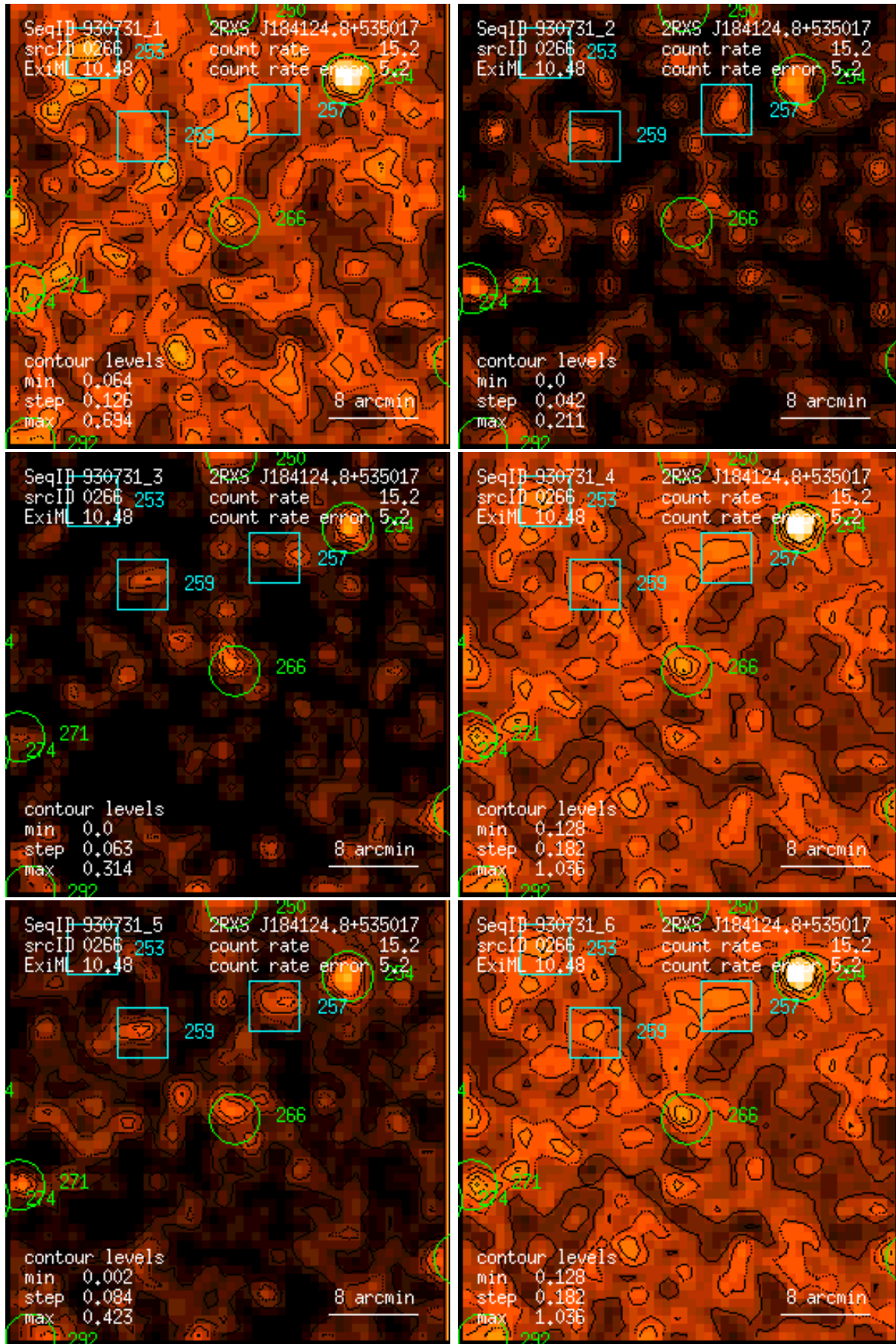
Figure 266: RASS 930731: detection 0266: band rate images, Gaussian filter: (1) PSPC channels 11 – 41, (2) 52 – 90, (3) 91 – 201, (4) 11 – 235, (5) 52 – 201, (6) 11 – 201. Broad band rates in counts/ks. Band rate contour levels in counts/ks/arcmin 2 .
