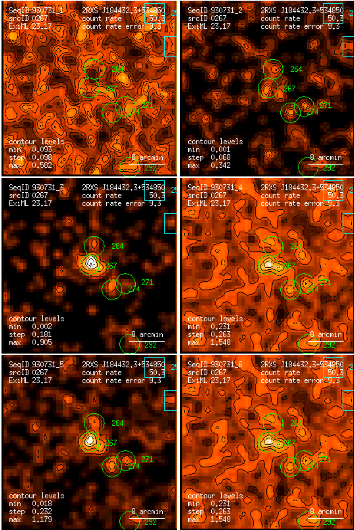
Figure 267: RASS 930731: detection 0267: band rate images, Gaussian filter: (1) PSPC channels 11 – 41, (2) 52 – 90, (3) 91 – 201, (4) 11 – 235, (5) 52 – 201, (6) 11 – 201. Broad band rates in counts/ks. Band rate contour levels in counts/ks/arcmin 2 .
