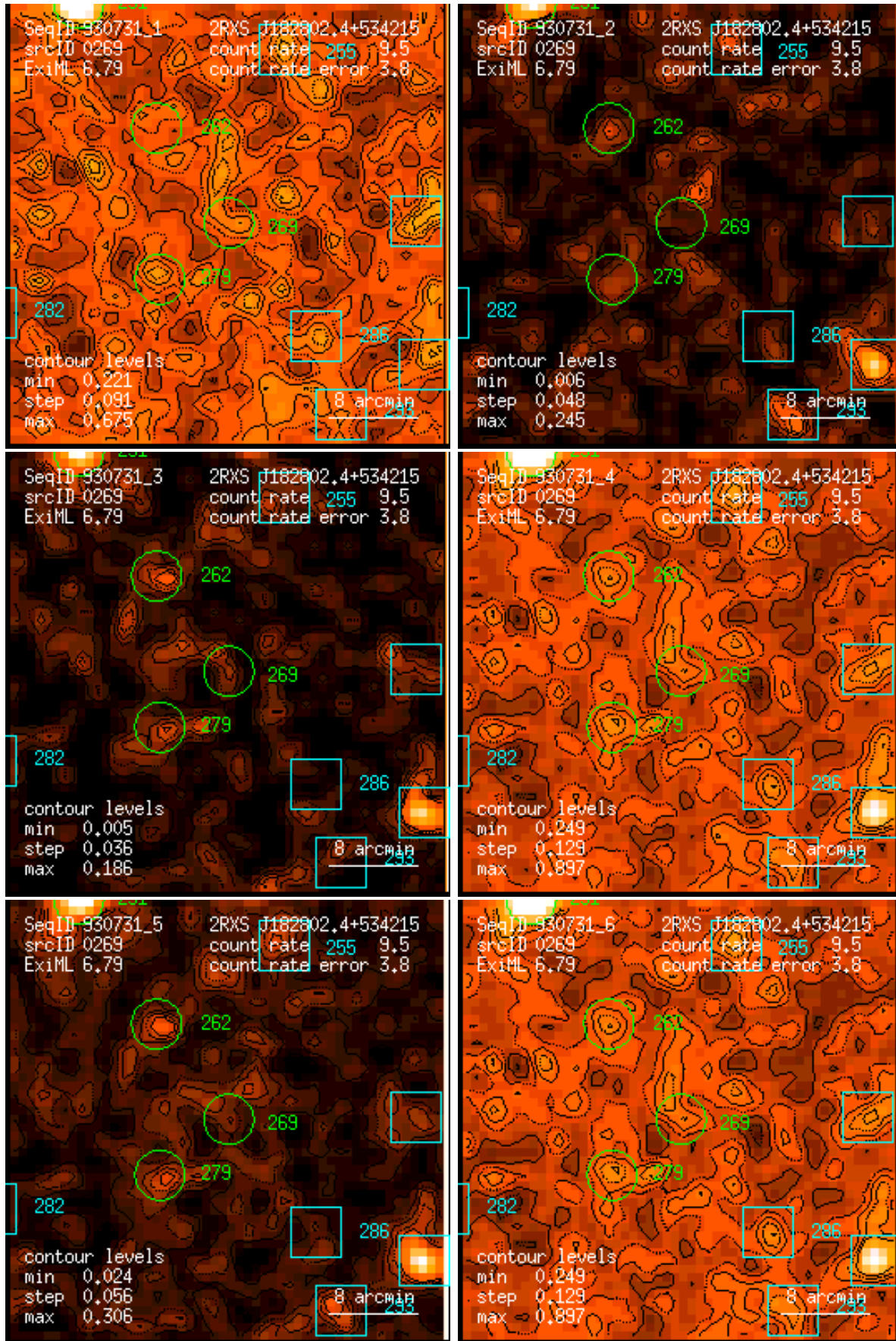
Figure 269: RASS 930731: detection 0269: band rate images, Gaussian filter: (1) PSPC channels 11 – 41, (2) 52 – 90, (3) 91 – 201, (4) 11 – 235, (5) 52 – 201, (6) 11 – 201. Broad band rates in counts/ks. Band rate contour levels in counts/ks/arcmin 2 .
