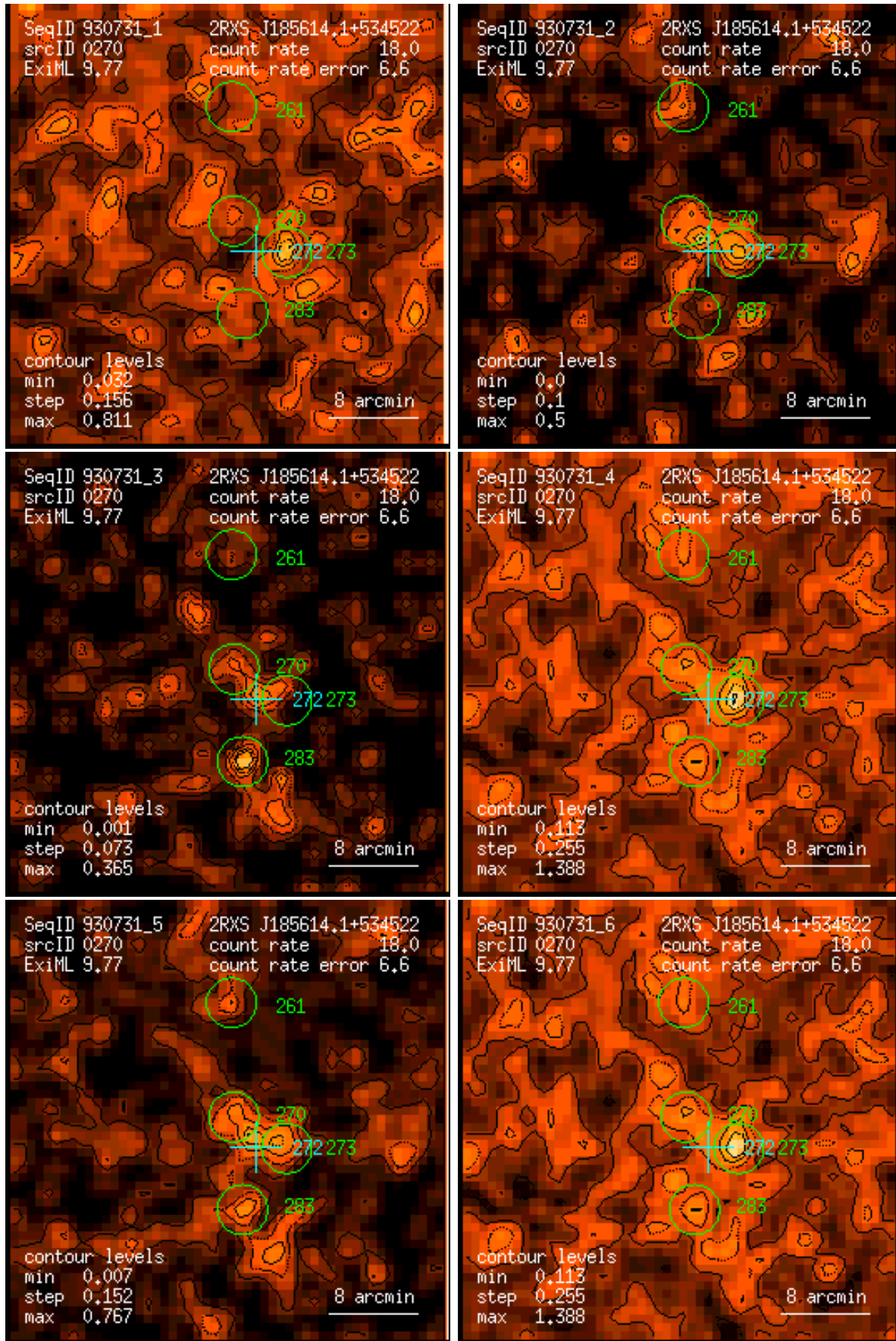
Figure 270: RASS 930731: detection 0270: band rate images, Gaussian filter: (1) PSPC channels 11 – 41, (2) 52 – 90, (3) 91 – 201, (4) 11 – 235, (5) 52 – 201, (6) 11 – 201. Broad band rates in counts/ks. Band rate contour levels in counts/ks/arcmin 2 .
