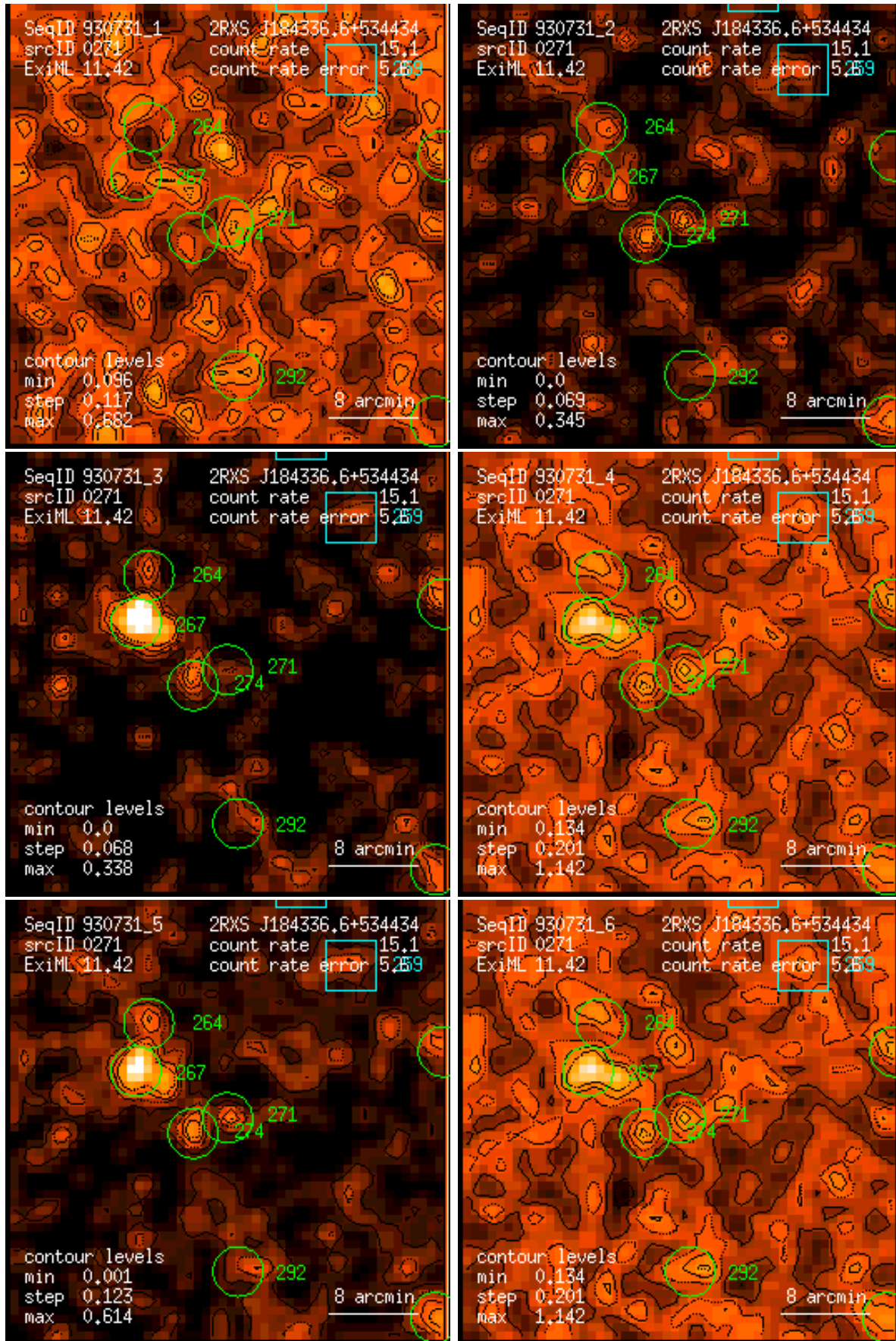
Figure 271: RASS 930731: detection 0271: band rate images, Gaussian filter: (1) PSPC channels 11 – 41, (2) 52 – 90, (3) 91 – 201, (4) 11 – 235, (5) 52 – 201, (6) 11 – 201. Broad band rates in counts/ks. Band rate contour levels in counts/ks/arcmin 2 .
