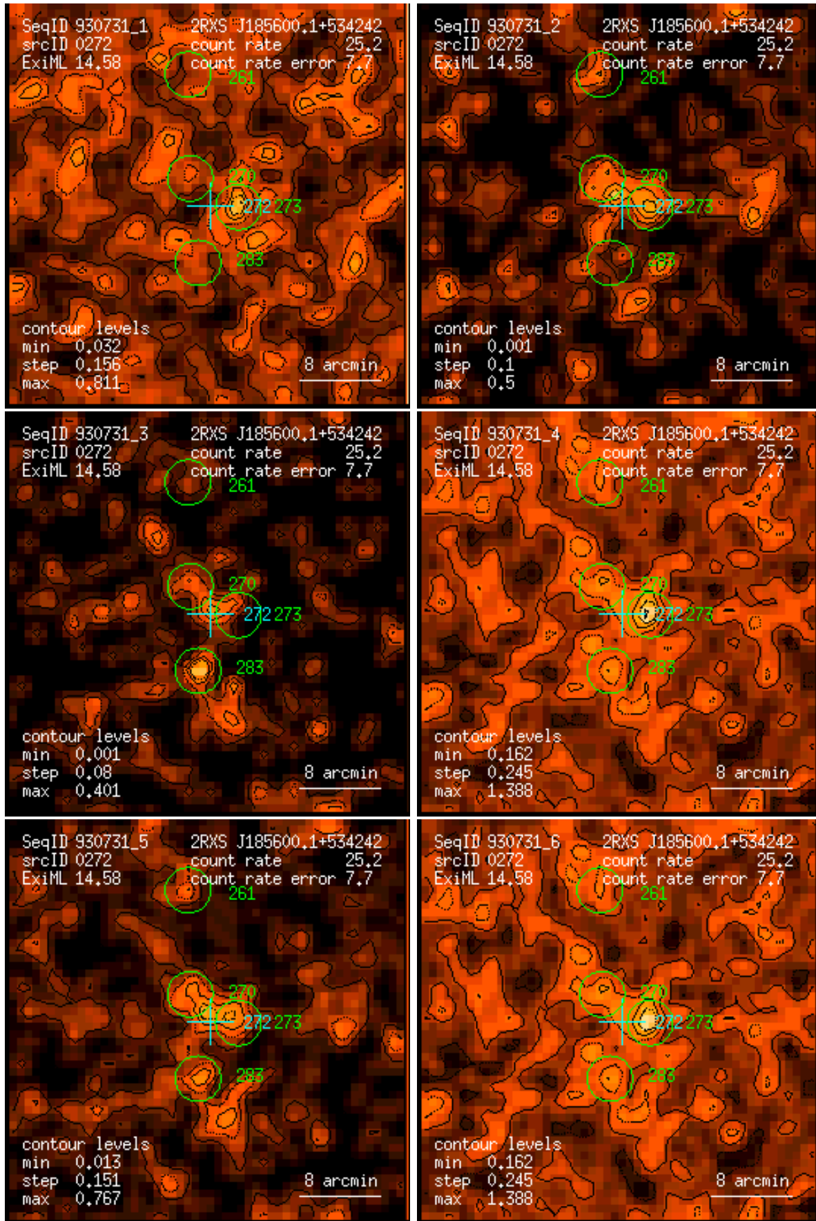
Figure 272: RASS 930731: detection 0272: band rate images, Gaussian filter: (1) PSPC channels 11 – 41, (2) 52 – 90, (3) 91 – 201, (4) 11 – 235, (5) 52 – 201, (6) 11 – 201. Broad band rates in counts/ks. Band rate contour levels in counts/ks/arcmin 2 .
