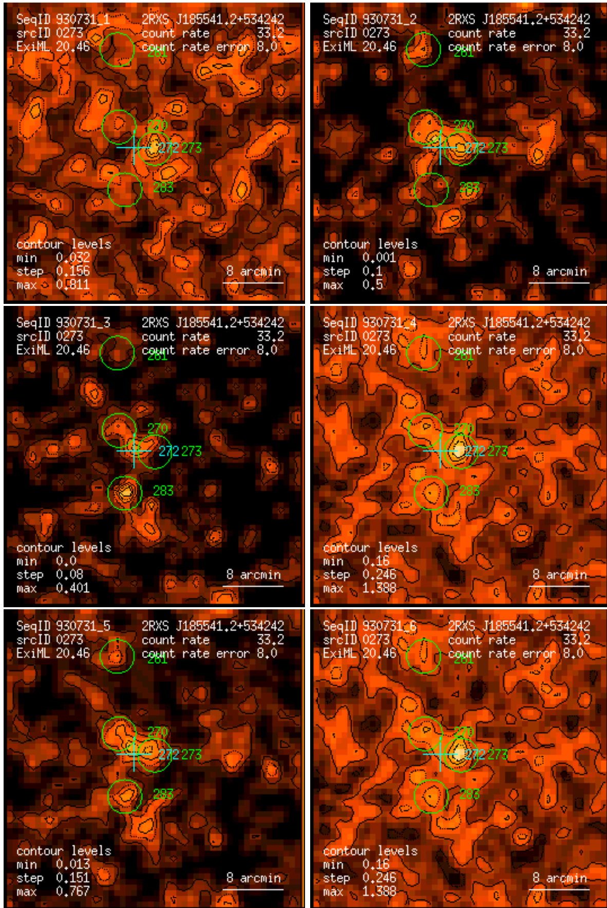
Figure 273: RASS 930731: detection 0273: band rate images, Gaussian filter: (1) PSPC channels 11 – 41, (2) 52 – 90, (3) 91 – 201, (4) 11 – 235, (5) 52 – 201, (6) 11 – 201. Broad band rates in counts/ks. Band rate contour levels in counts/ks/arcmin 2 .
