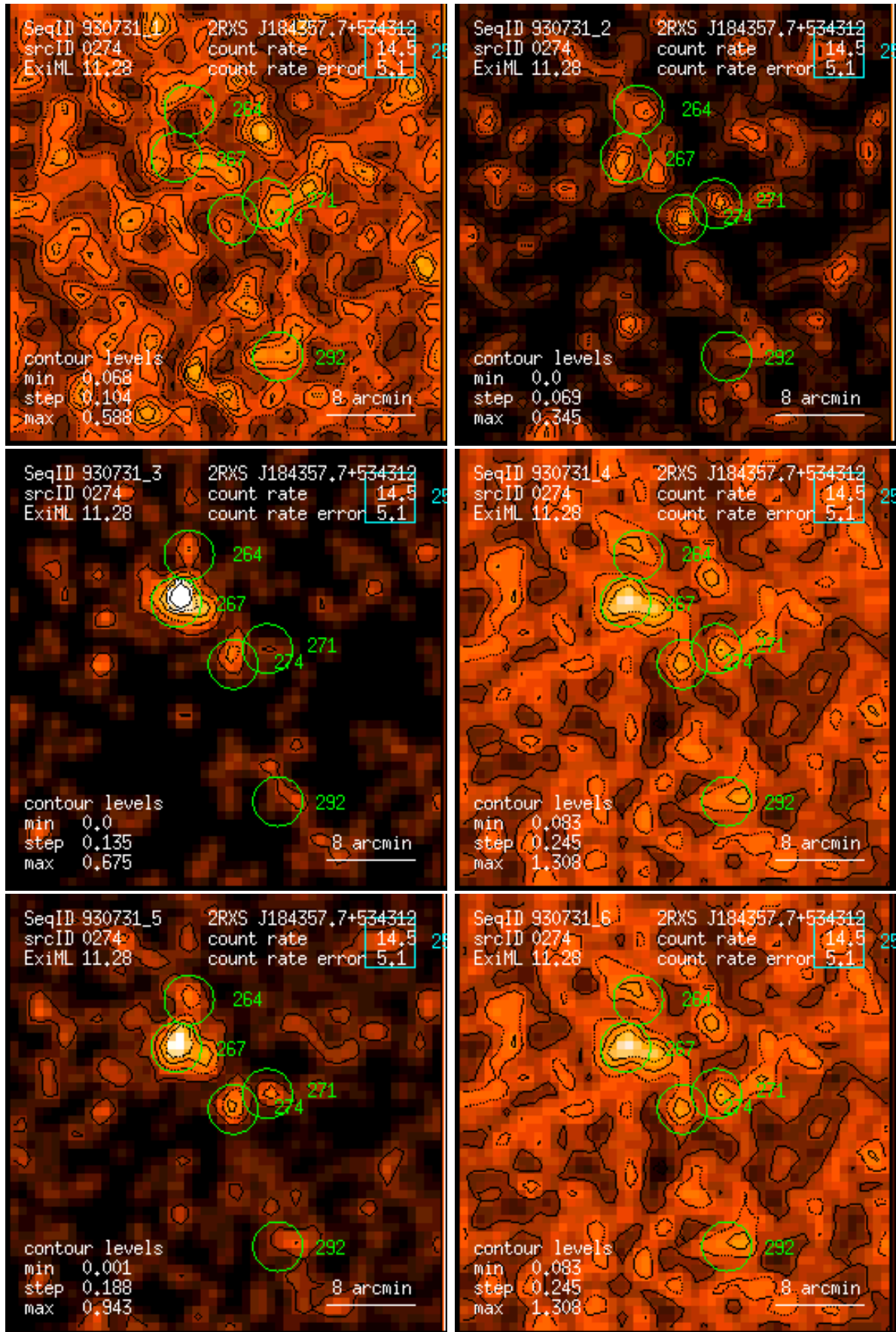
Figure 274: RASS 930731: detection 0274: band rate images, Gaussian filter: (1) PSPC channels 11 – 41, (2) 52 – 90, (3) 91 – 201, (4) 11 – 235, (5) 52 – 201, (6) 11 – 201. Broad band rates in counts/ks. Band rate contour levels in counts/ks/arcmin 2 .
