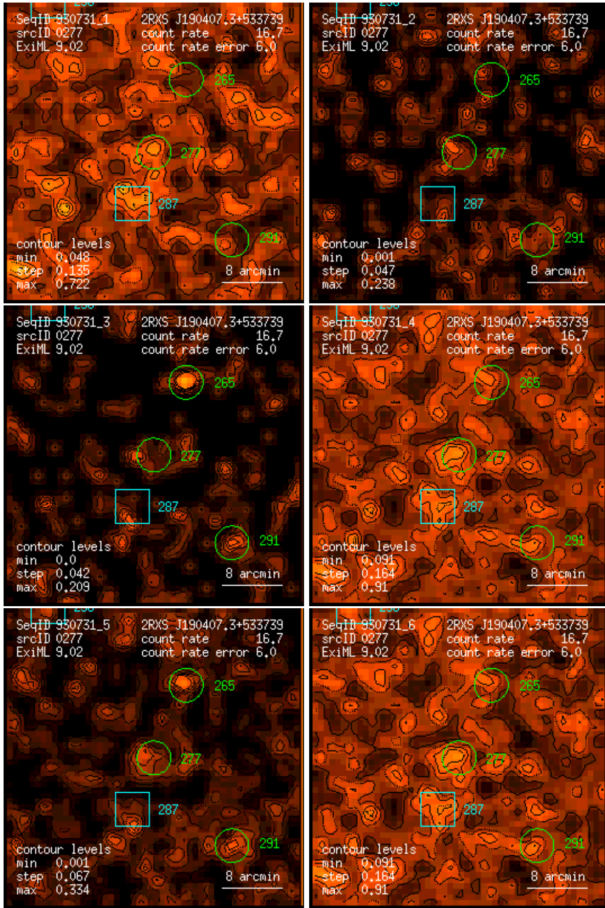
Figure 277: RASS 930731: detection 0277: band rate images, Gaussian filter: (1) PSPC channels 11 – 41, (2) 52 – 90, (3) 91 – 201, (4) 11 – 235, (5) 52 – 201, (6) 11 – 201. Broad band rates in counts/ks. Band rate contour levels in counts/ks/arcmin 2 .
