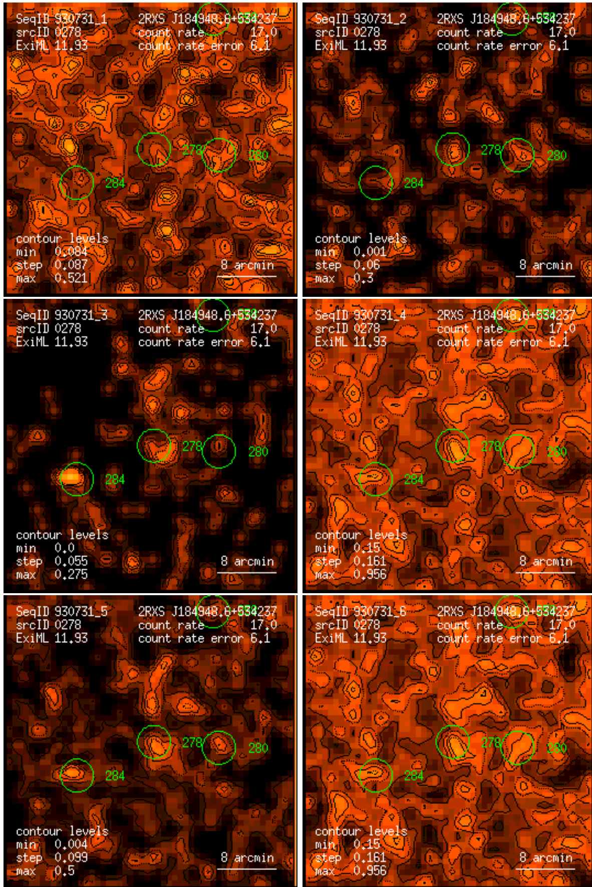
Figure 278: RASS 930731: detection 0278: band rate images, Gaussian filter: (1) PSPC channels 11 – 41, (2) 52 – 90, (3) 91 – 201, (4) 11 – 235, (5) 52 – 201, (6) 11 – 201. Broad band rates in counts/ks. Band rate contour levels in counts/ks/arcmin 2 .
