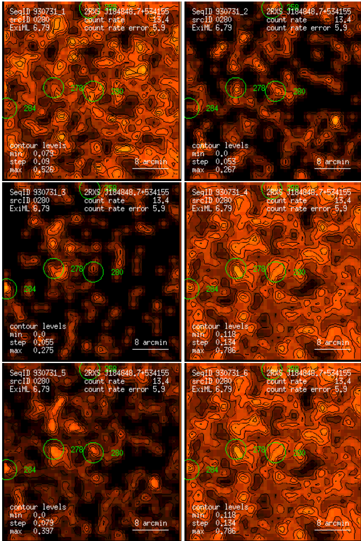
Figure 280: RASS 930731: detection 0280: band rate images, Gaussian filter: (1) PSPC channels 11 – 41, (2) 52 – 90, (3) 91 – 201, (4) 11 – 235, (5) 52 – 201, (6) 11 – 201. Broad band rates in counts/ks. Band rate contour levels in counts/ks/arcmin 2 .
