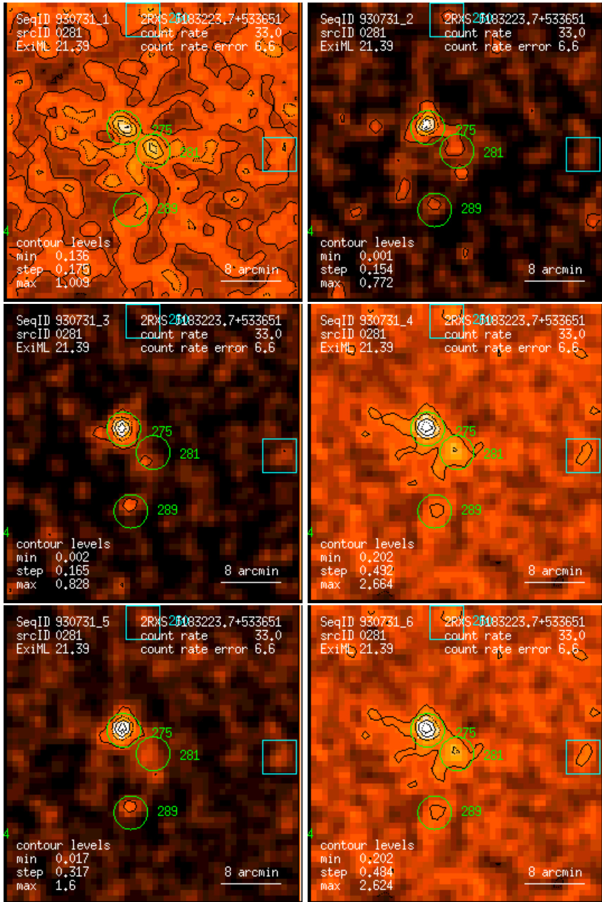
Figure 281: RASS 930731: detection 0281: band rate images, Gaussian filter: (1) PSPC channels 11 – 41, (2) 52 – 90, (3) 91 – 201, (4) 11 – 235, (5) 52 – 201, (6) 11 – 201. Broad band rates in counts/ks. Band rate contour levels in counts/ks/arcmin 2 .
