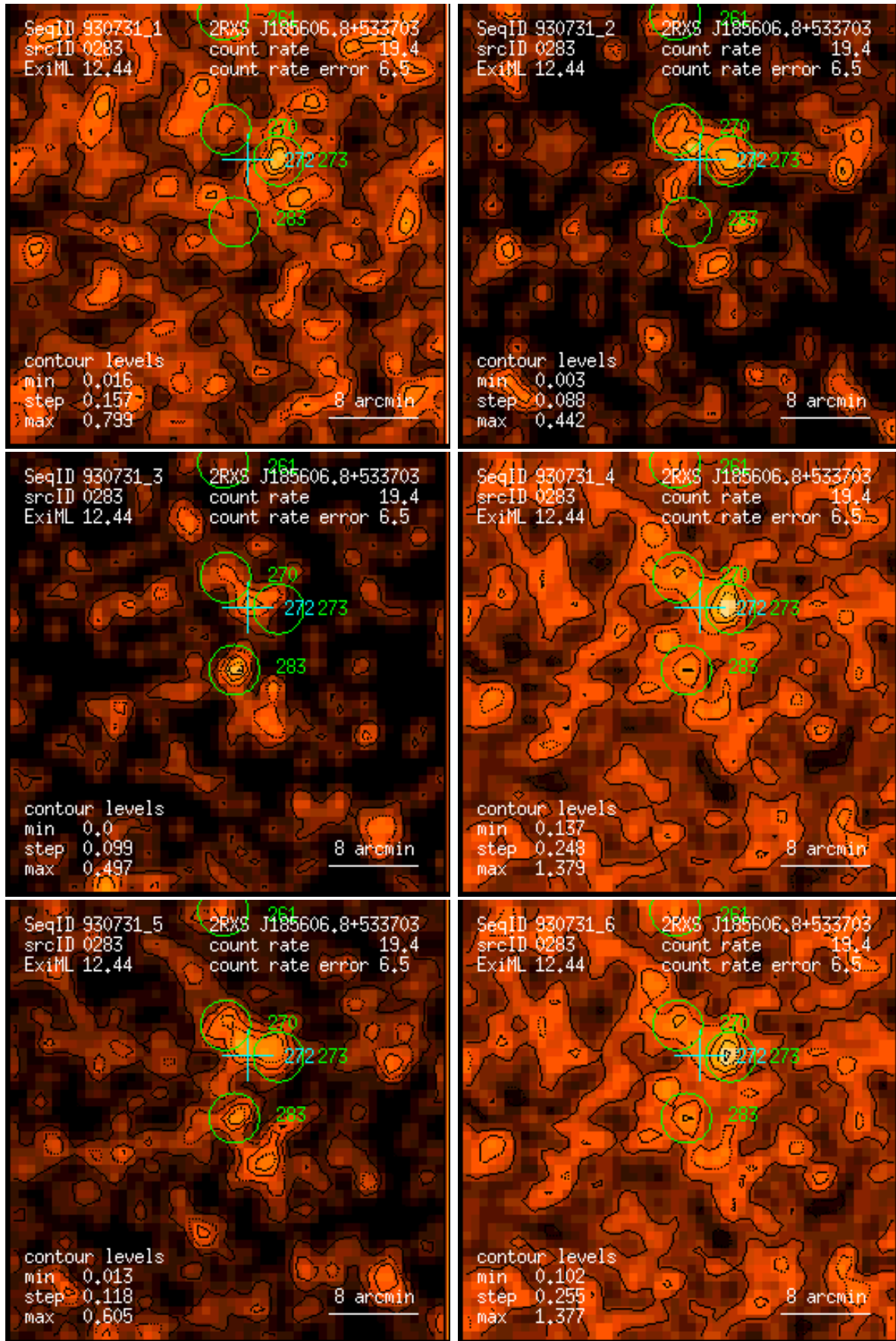
Figure 283: RASS 930731: detection 0283: band rate images, Gaussian filter: (1) PSPC channels 11 – 41, (2) 52 – 90, (3) 91 – 201, (4) 11 – 235, (5) 52 – 201, (6) 11 – 201. Broad band rates in counts/ks. Band rate contour levels in counts/ks/arcmin 2 .
