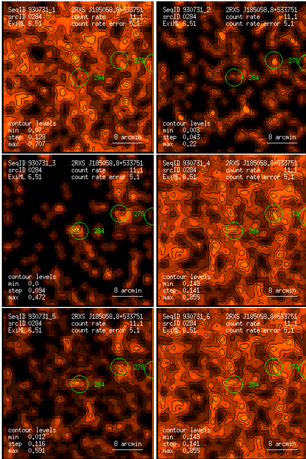
Figure 284: RASS 930731: detection 0284: band rate images, Gaussian filter: (1) PSPC channels 11 – 41, (2) 52 – 90, (3) 91 – 201, (4) 11 – 235, (5) 52 – 201, (6) 11 – 201. Broad band rates in counts/ks. Band rate contour levels in counts/ks/arcmin 2 .
