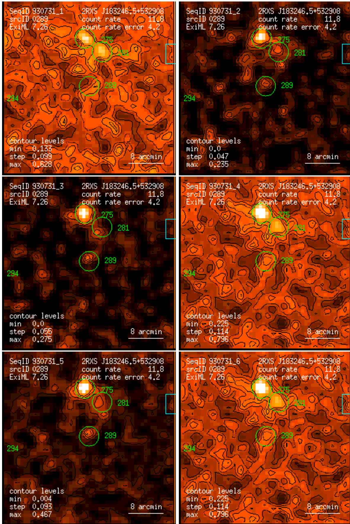
Figure 289: RASS 930731: detection 0289: band rate images, Gaussian filter: (1) PSPC channels 11 – 41, (2) 52 – 90, (3) 91 – 201, (4) 11 – 235, (5) 52 – 201, (6) 11 – 201. Broad band rates in counts/ks. Band rate contour levels in counts/ks/arcmin 2 .
