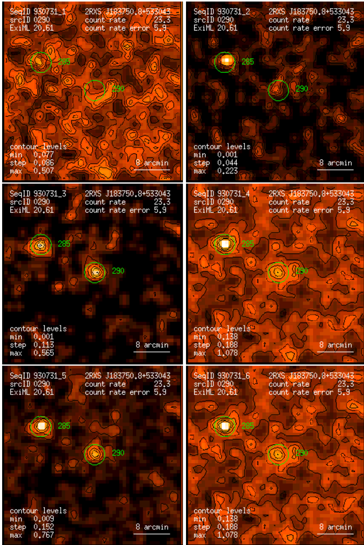
Figure 290: RASS 930731: detection 0290: band rate images, Gaussian filter: (1) PSPC channels 11 – 41, (2) 52 – 90, (3) 91 – 201, (4) 11 – 235, (5) 52 – 201, (6) 11 – 201. Broad band rates in counts/ks. Band rate contour levels in counts/ks/arcmin 2 .
