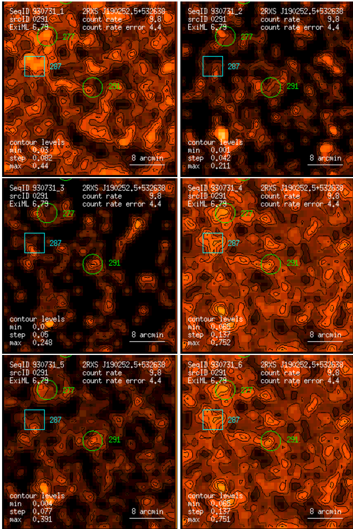
Figure 291: RASS 930731: detection 0291: band rate images, Gaussian filter: (1) PSPC channels 11 – 41, (2) 52 – 90, (3) 91 – 201, (4) 11 – 235, (5) 52 – 201, (6) 11 – 201. Broad band rates in counts/ks. Band rate contour levels in counts/ks/arcmin 2 .
