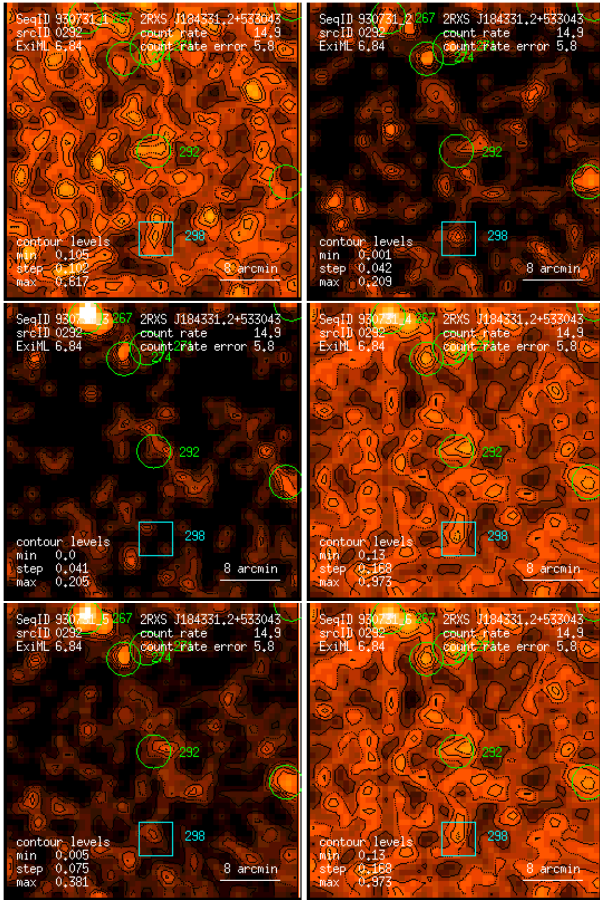
Figure 292: RASS 930731: detection 0292: band rate images, Gaussian filter: (1) PSPC channels 11 – 41, (2) 52 – 90, (3) 91 – 201, (4) 11 – 235, (5) 52 – 201, (6) 11 – 201. Broad band rates in counts/ks. Band rate contour levels in counts/ks/arcmin 2 .
