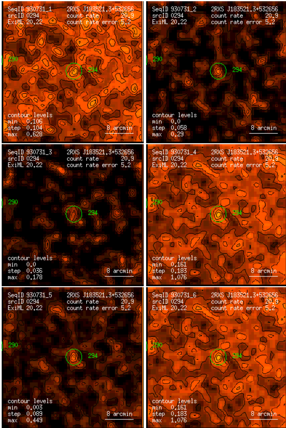
Figure 294: RASS 930731: detection 0294: band rate images, Gaussian filter: (1) PSPC channels 11 – 41, (2) 52 – 90, (3) 91 – 201, (4) 11 – 235, (5) 52 – 201, (6) 11 – 201. Broad band rates in counts/ks. Band rate contour levels in counts/ks/arcmin 2 .
