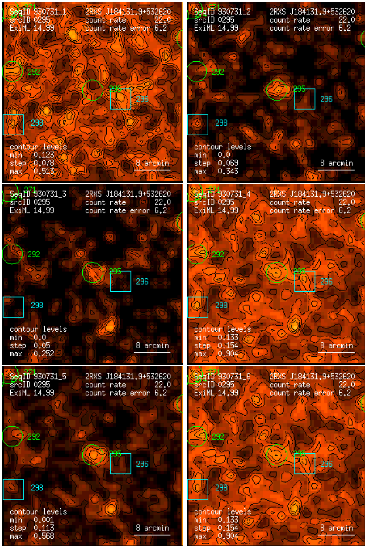
Figure 295: RASS 930731: detection 0295: band rate images, Gaussian filter: (1) PSPC channels 11 – 41, (2) 52 – 90, (3) 91 – 201, (4) 11 – 235, (5) 52 – 201, (6) 11 – 201. Broad band rates in counts/ks. Band rate contour levels in counts/ks/arcmin 2 .
