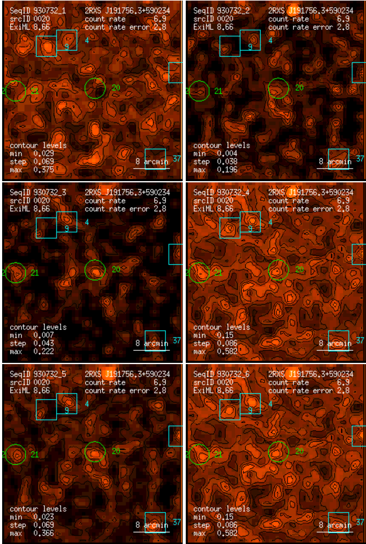
Figure 20: RASS 930732: detection 0020: band rate images, Gaussian filter: (1) PSPC channels 11 – 41, (2) 52 – 90, (3) 91 – 201, (4) 11 – 235, (5) 52 – 201, (6) 11 – 201. Broad band rates in counts/ks. Band rate contour levels in counts/ks/arcmin 2 .
