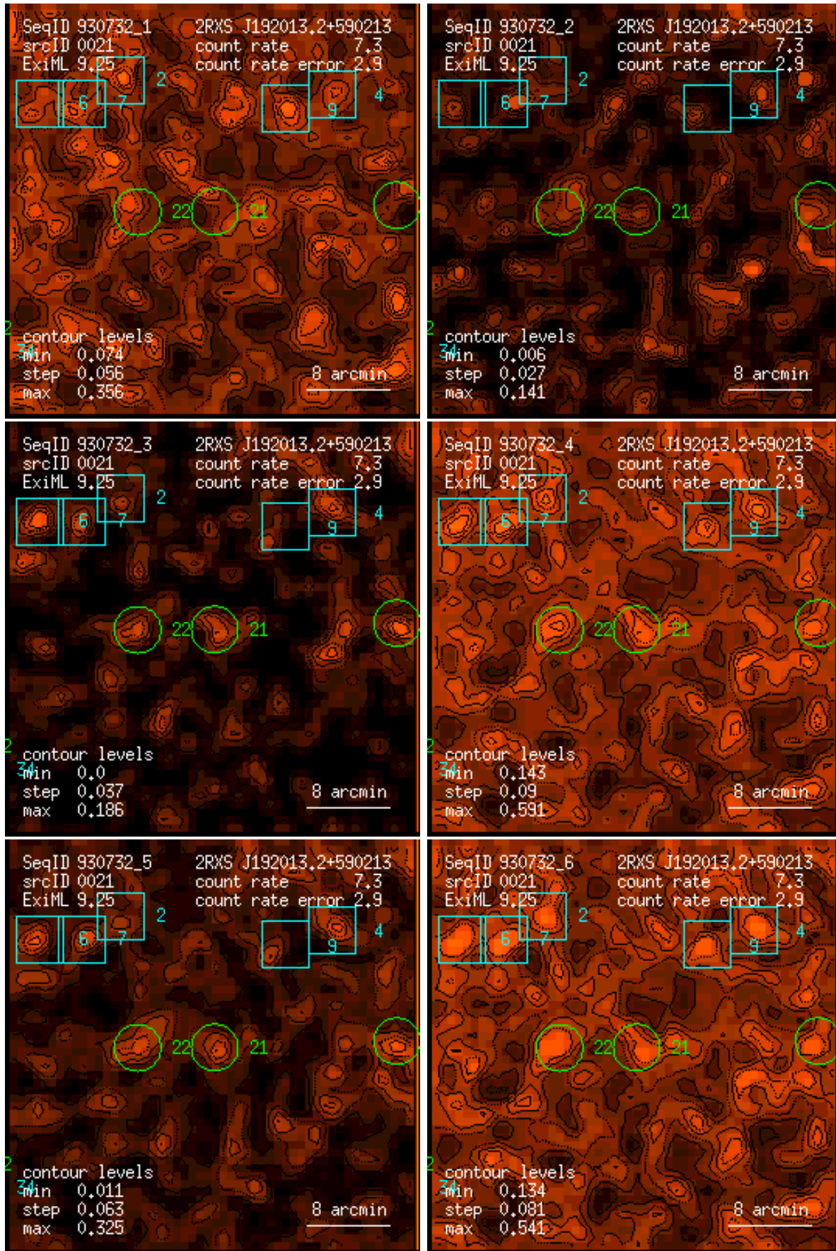
Figure 21: RASS 930732: detection 0021: band rate images, Gaussian filter: (1) PSPC channels 11 – 41, (2) 52 – 90, (3) 91 – 201, (4) 11 – 235, (5) 52 – 201, (6) 11 – 201. Broad band rates in counts/ks. Band rate contour levels in counts/ks/arcmin 2 .
