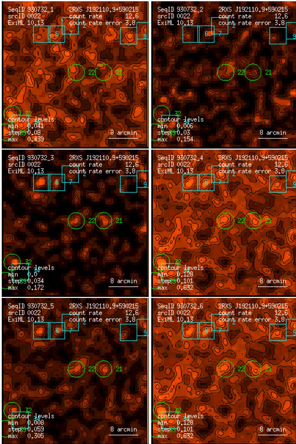
Figure 22: RASS 930732: detection 0022: band rate images, Gaussian filter: (1) PSPC channels 11 – 41, (2) 52 – 90, (3) 91 – 201, (4) 11 – 235, (5) 52 – 201, (6) 11 – 201. Broad band rates in counts/ks. Band rate contour levels in counts/ks/arcmin 2 .
