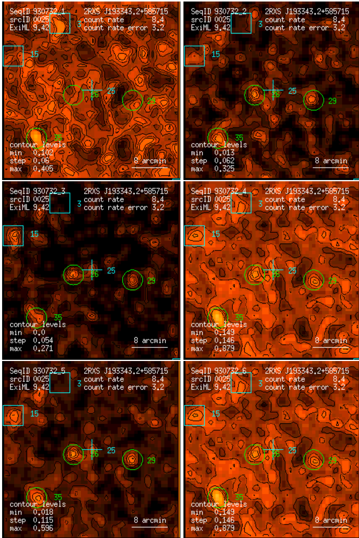
Figure 25: RASS 930732: detection 0025: band rate images, Gaussian filter: (1) PSPC channels 11 – 41, (2) 52 – 90, (3) 91 – 201, (4) 11 – 235, (5) 52 – 201, (6) 11 – 201. Broad band rates in counts/ks. Band rate contour levels in counts/ks/arcmin 2 .
