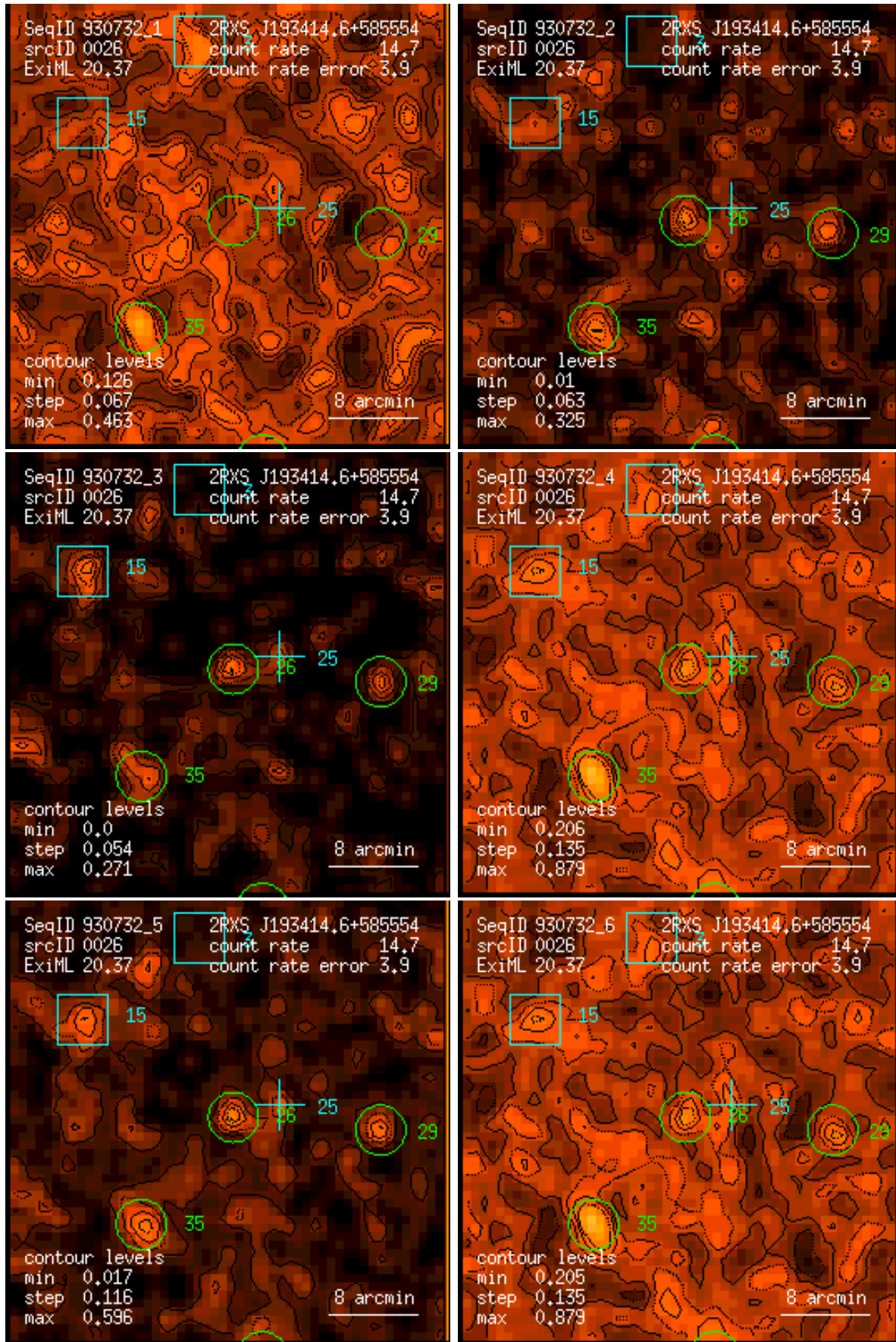
Figure 26: RASS 930732: detection 0026: band rate images, Gaussian filter: (1) PSPC channels 11 – 41, (2) 52 – 90, (3) 91 – 201, (4) 11 – 235, (5) 52 – 201, (6) 11 – 201. Broad band rates in counts/ks. Band rate contour levels in counts/ks/arcmin 2 .
