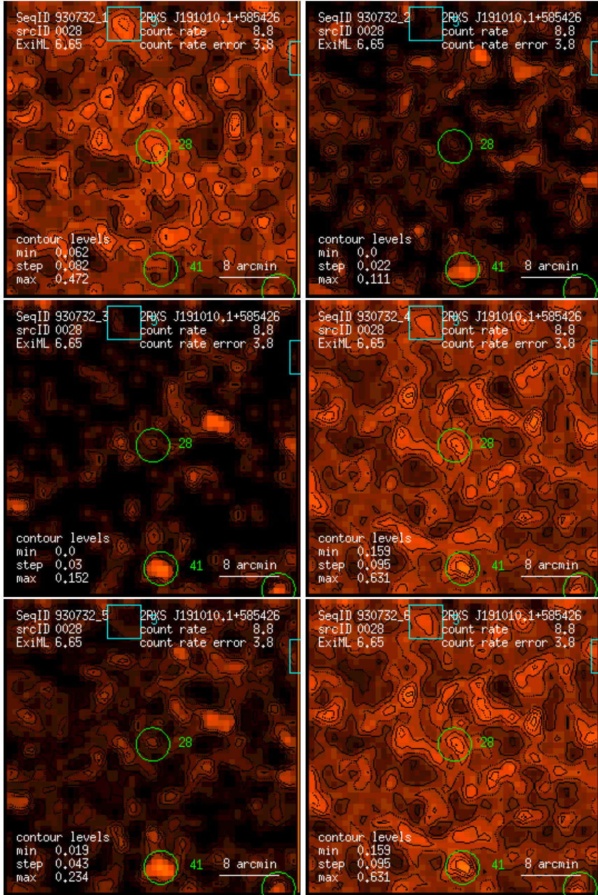
Figure 28: RASS 930732: detection 0028: band rate images, Gaussian filter: (1) PSPC channels 11 – 41, (2) 52 – 90, (3) 91 – 201, (4) 11 – 235, (5) 52 – 201, (6) 11 – 201. Broad band rates in counts/ks. Band rate contour levels in counts/ks/arcmin 2 .
