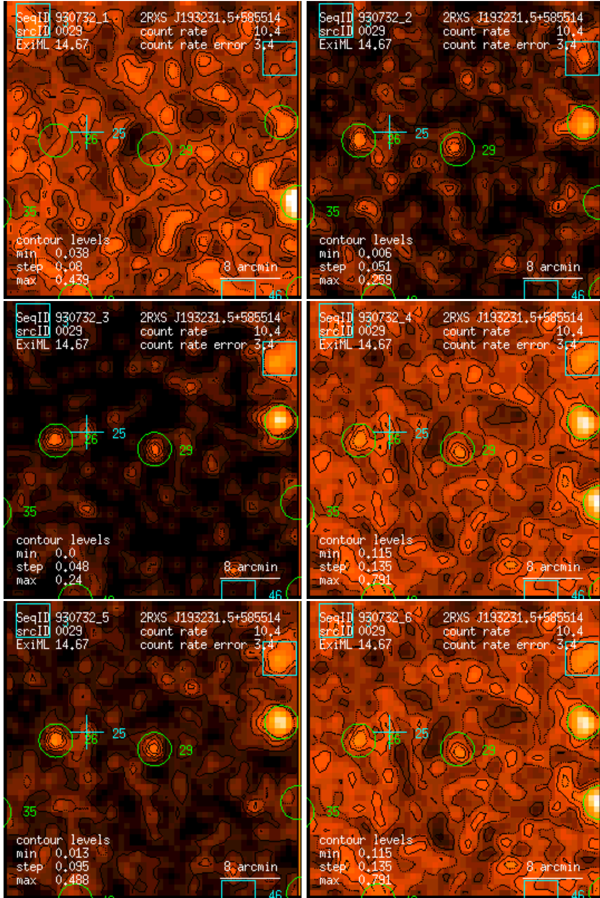
Figure 29: RASS 930732: detection 0029: band rate images, Gaussian filter: (1) PSPC channels 11 – 41, (2) 52 – 90, (3) 91 – 201, (4) 11 – 235, (5) 52 – 201, (6) 11 – 201. Broad band rates in counts/ks. Band rate contour levels in counts/ks/arcmin 2 .
