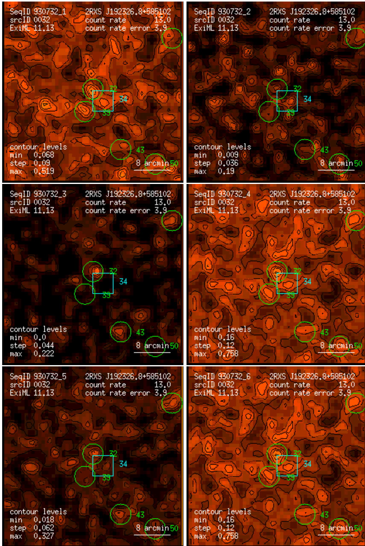
Figure 32: RASS 930732: detection 0032: band rate images, Gaussian filter: (1) PSPC channels 11 – 41, (2) 52 – 90, (3) 91 – 201, (4) 11 – 235, (5) 52 – 201, (6) 11 – 201. Broad band rates in counts/ks. Band rate contour levels in counts/ks/arcmin 2 .
