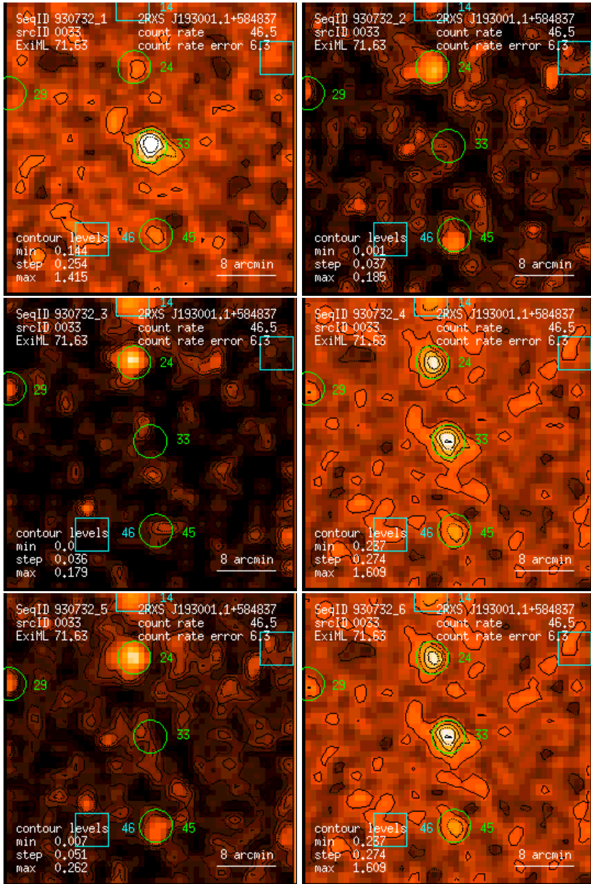
Figure 33: RASS 930732: detection 0033: band rate images, Gaussian filter: (1) PSPC channels 11 – 41, (2) 52 – 90, (3) 91 – 201, (4) 11 – 235, (5) 52 – 201, (6) 11 – 201. Broad band rates in counts/ks. Band rate contour levels in counts/ks/arcmin 2 .
