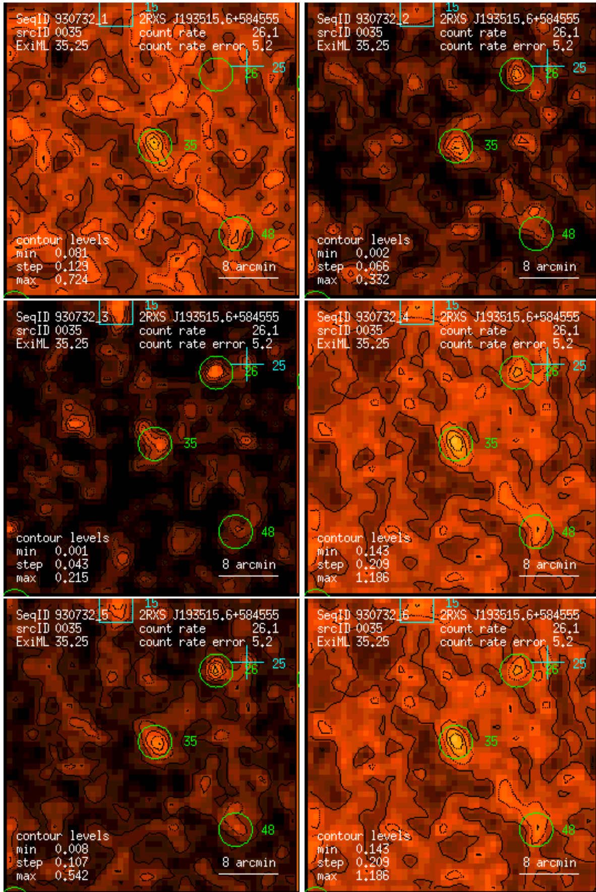
Figure 35: RASS 930732: detection 0035: band rate images, Gaussian filter: (1) PSPC channels 11 – 41, (2) 52 – 90, (3) 91 – 201, (4) 11 – 235, (5) 52 – 201, (6) 11 – 201. Broad band rates in counts/ks. Band rate contour levels in counts/ks/arcmin 2 .
