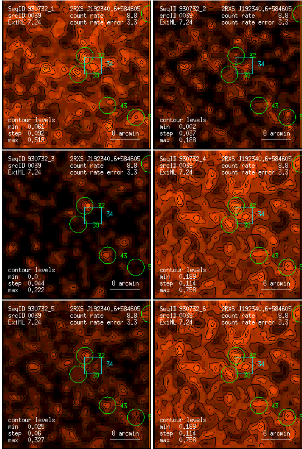
Figure 39: RASS 930732: detection 0039: band rate images, Gaussian filter: (1) PSPC channels 11 – 41, (2) 52 – 90, (3) 91 – 201, (4) 11 – 235, (5) 52 – 201, (6) 11 – 201. Broad band rates in counts/ks. Band rate contour levels in counts/ks/arcmin 2 .
