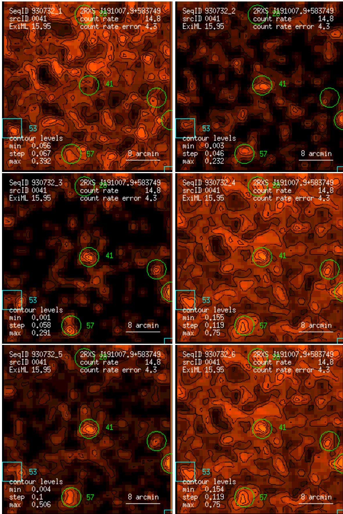
Figure 41: RASS 930732: detection 0041: band rate images, Gaussian filter: (1) PSPC channels 11 – 41, (2) 52 – 90, (3) 91 – 201, (4) 11 – 235, (5) 52 – 201, (6) 11 – 201. Broad band rates in counts/ks. Band rate contour levels in counts/ks/arcmin 2 .
