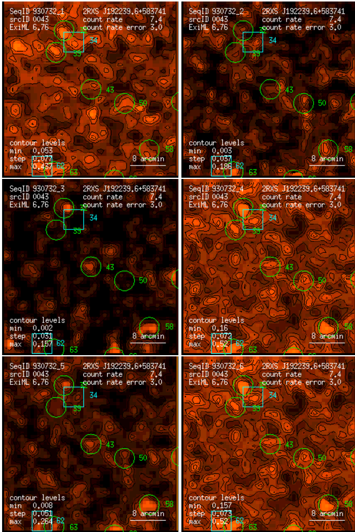
Figure 43: RASS 930732: detection 0043: band rate images, Gaussian filter: (1) PSPC channels 11 – 41, (2) 52 – 90, (3) 91 – 201, (4) 11 – 235, (5) 52 – 201, (6) 11 – 201. Broad band rates in counts/ks. Band rate contour levels in counts/ks/arcmin 2 .
