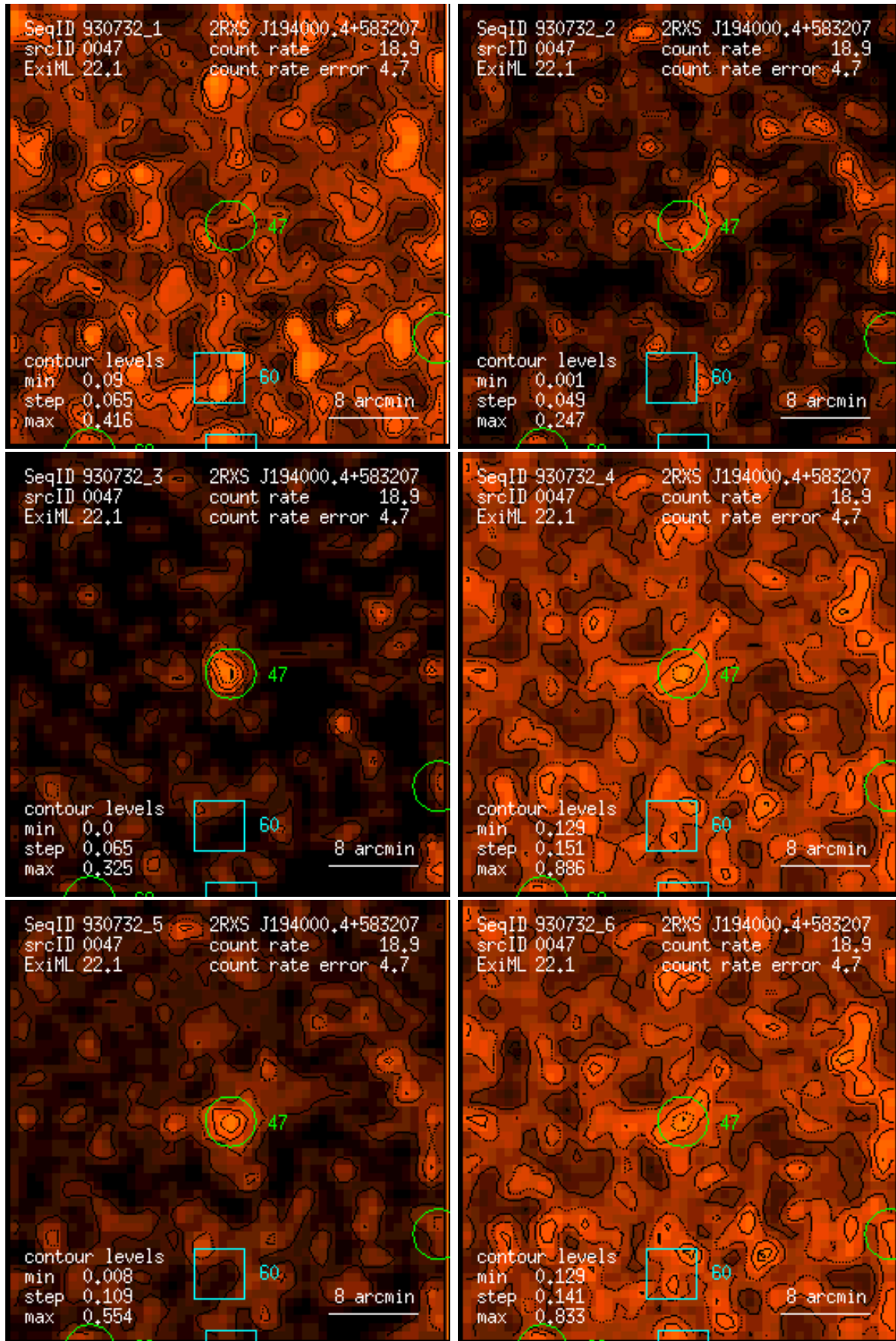
Figure 47: RASS 930732: detection 0047: band rate images, Gaussian filter: (1) PSPC channels 11 – 41, (2) 52 – 90, (3) 91 – 201, (4) 11 – 235, (5) 52 – 201, (6) 11 – 201. Broad band rates in counts/ks. Band rate contour levels in counts/ks/arcmin 2 .
