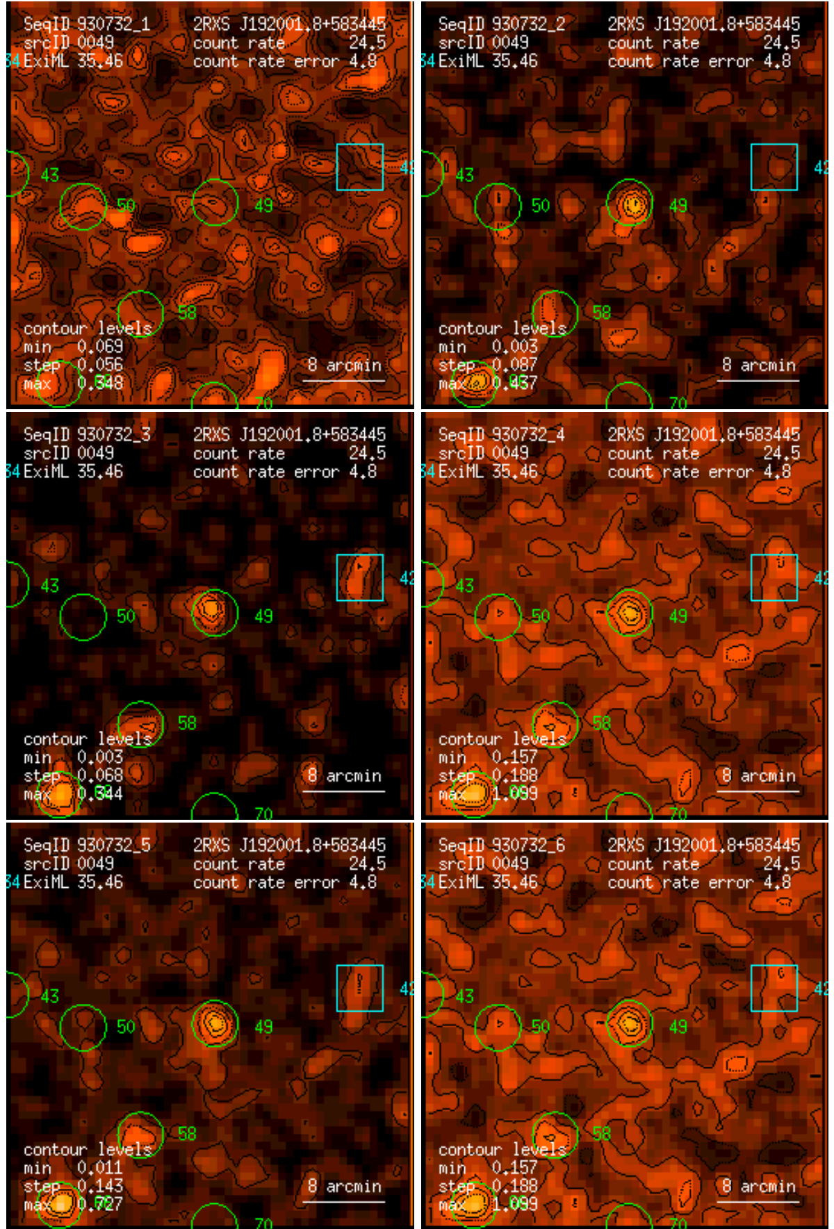
Figure 49: RASS 930732: detection 0049: band rate images, Gaussian filter: (1) PSPC channels 11 – 41, (2) 52 – 90, (3) 91 – 201, (4) 11 – 235, (5) 52 – 201, (6) 11 – 201. Broad band rates in counts/ks. Band rate contour levels in counts/ks/arcmin 2 .
