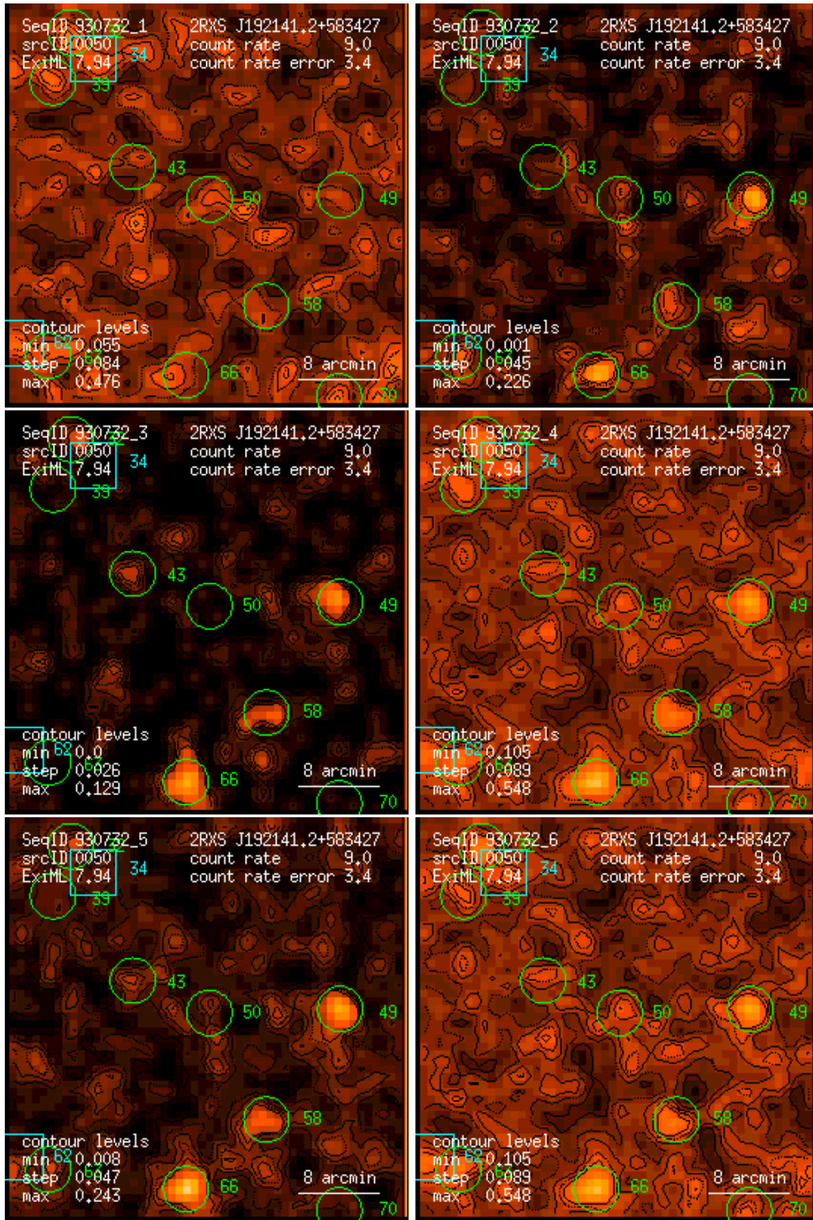
Figure 50: RASS 930732: detection 0050: band rate images, Gaussian filter: (1) PSPC channels 11 – 41, (2) 52 – 90, (3) 91 – 201, (4) 11 – 235, (5) 52 – 201, (6) 11 – 201. Broad band rates in counts/ks. Band rate contour levels in counts/ks/arcmin 2 .
