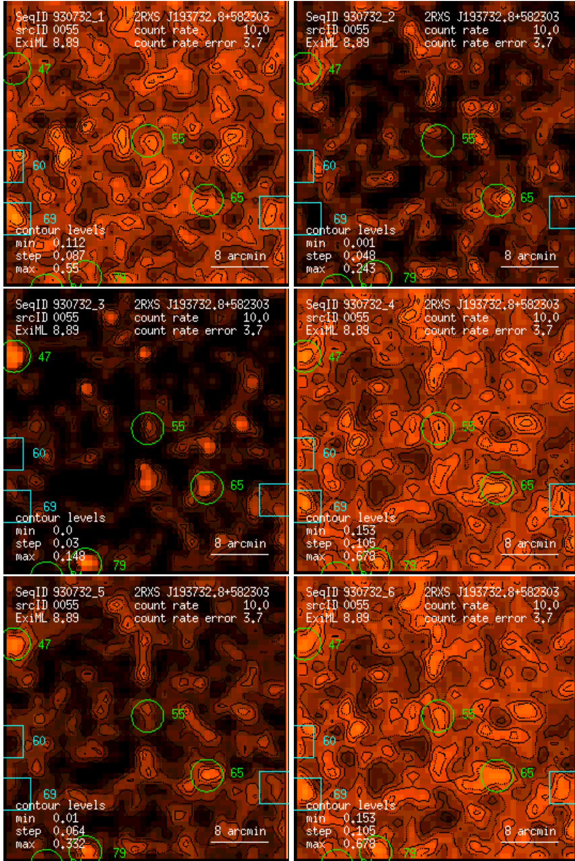
Figure 55: RASS 930732: detection 0055: band rate images, Gaussian filter: (1) PSPC channels 11 – 41, (2) 52 – 90, (3) 91 – 201, (4) 11 – 235, (5) 52 – 201, (6) 11 – 201. Broad band rates in counts/ks. Band rate contour levels in counts/ks/arcmin 2 .
