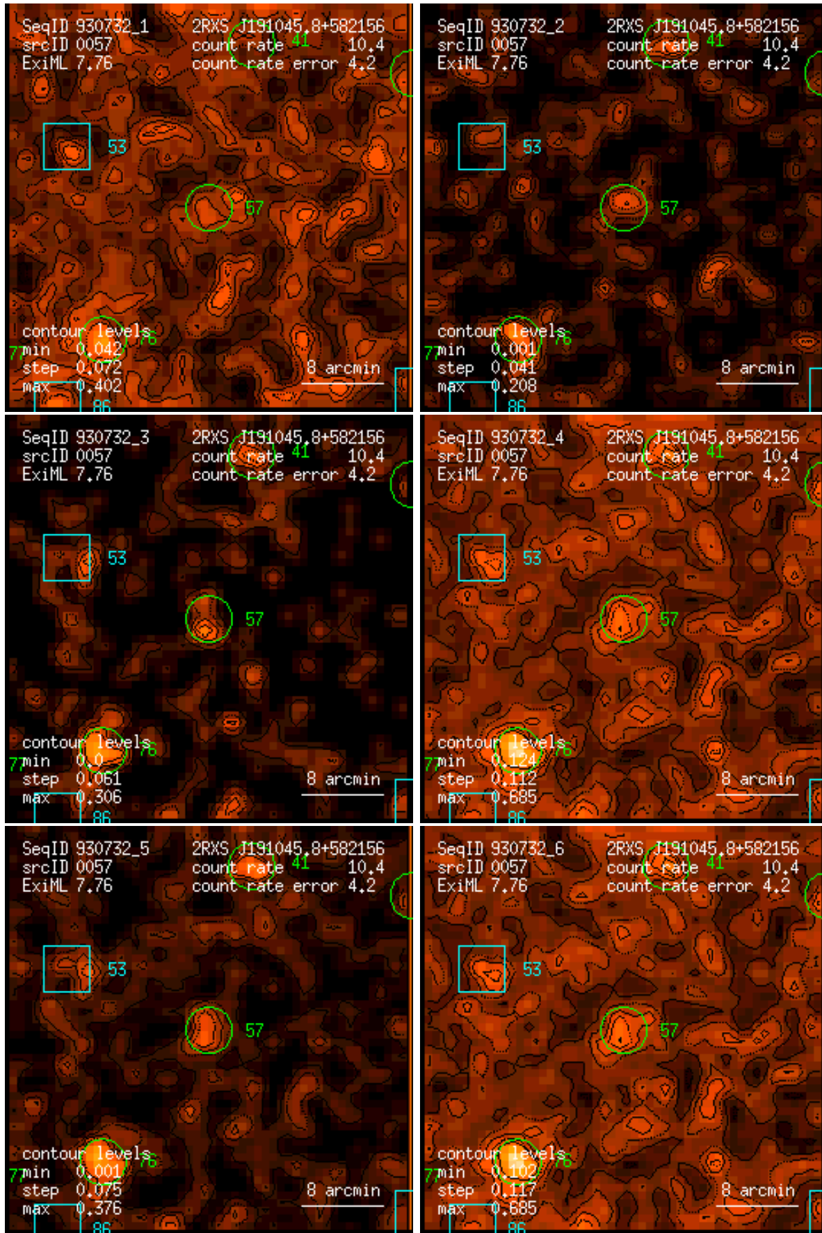
Figure 57: RASS 930732: detection 0057: band rate images, Gaussian filter: (1) PSPC channels 11 – 41, (2) 52 – 90, (3) 91 – 201, (4) 11 – 235, (5) 52 – 201, (6) 11 – 201. Broad band rates in counts/ks. Band rate contour levels in counts/ks/arcmin 2 .
