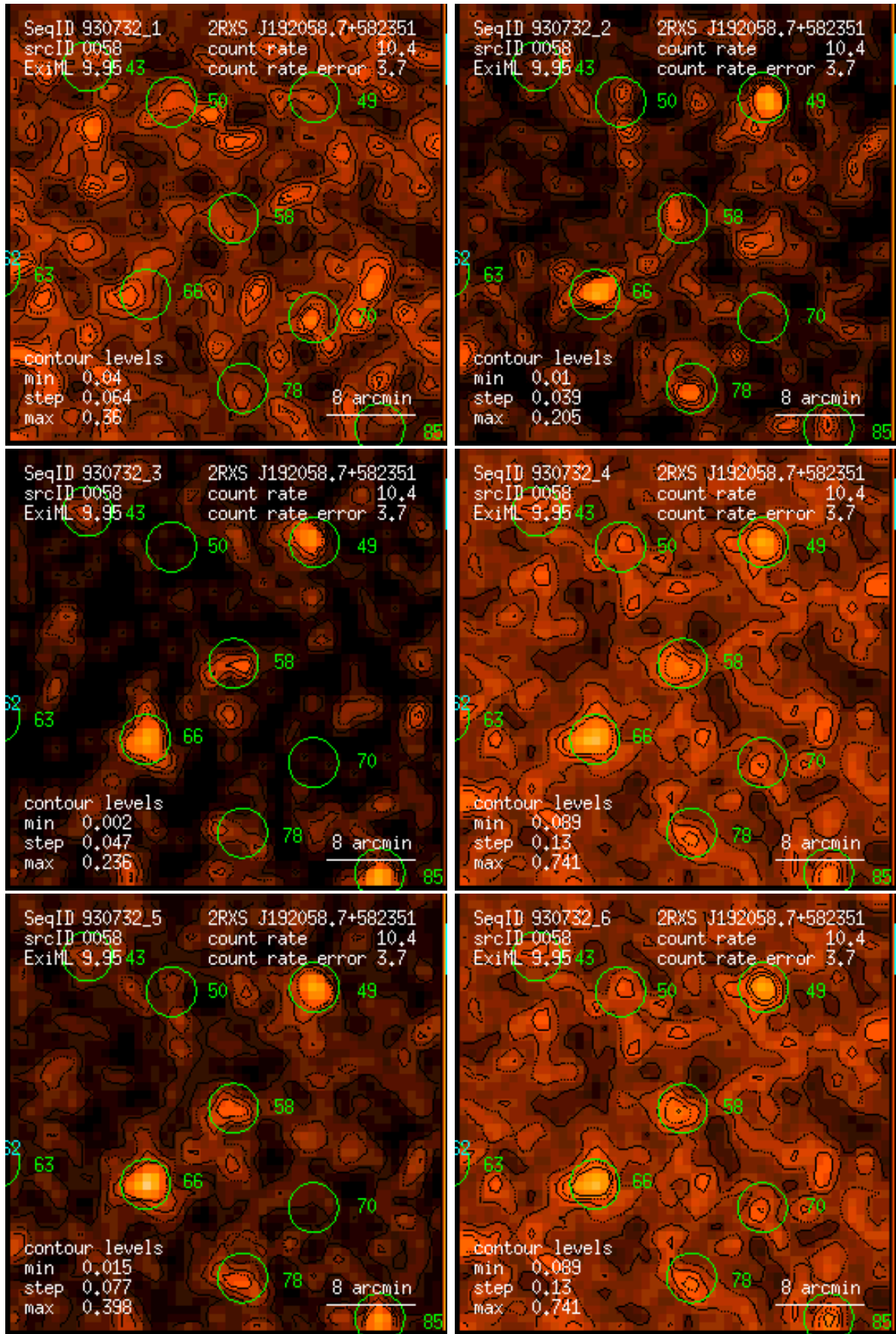
Figure 58: RASS 930732: detection 0058: band rate images, Gaussian filter: (1) PSPC channels 11 – 41, (2) 52 – 90, (3) 91 – 201, (4) 11 – 235, (5) 52 – 201, (6) 11 – 201. Broad band rates in counts/ks. Band rate contour levels in counts/ks/arcmin 2 .
