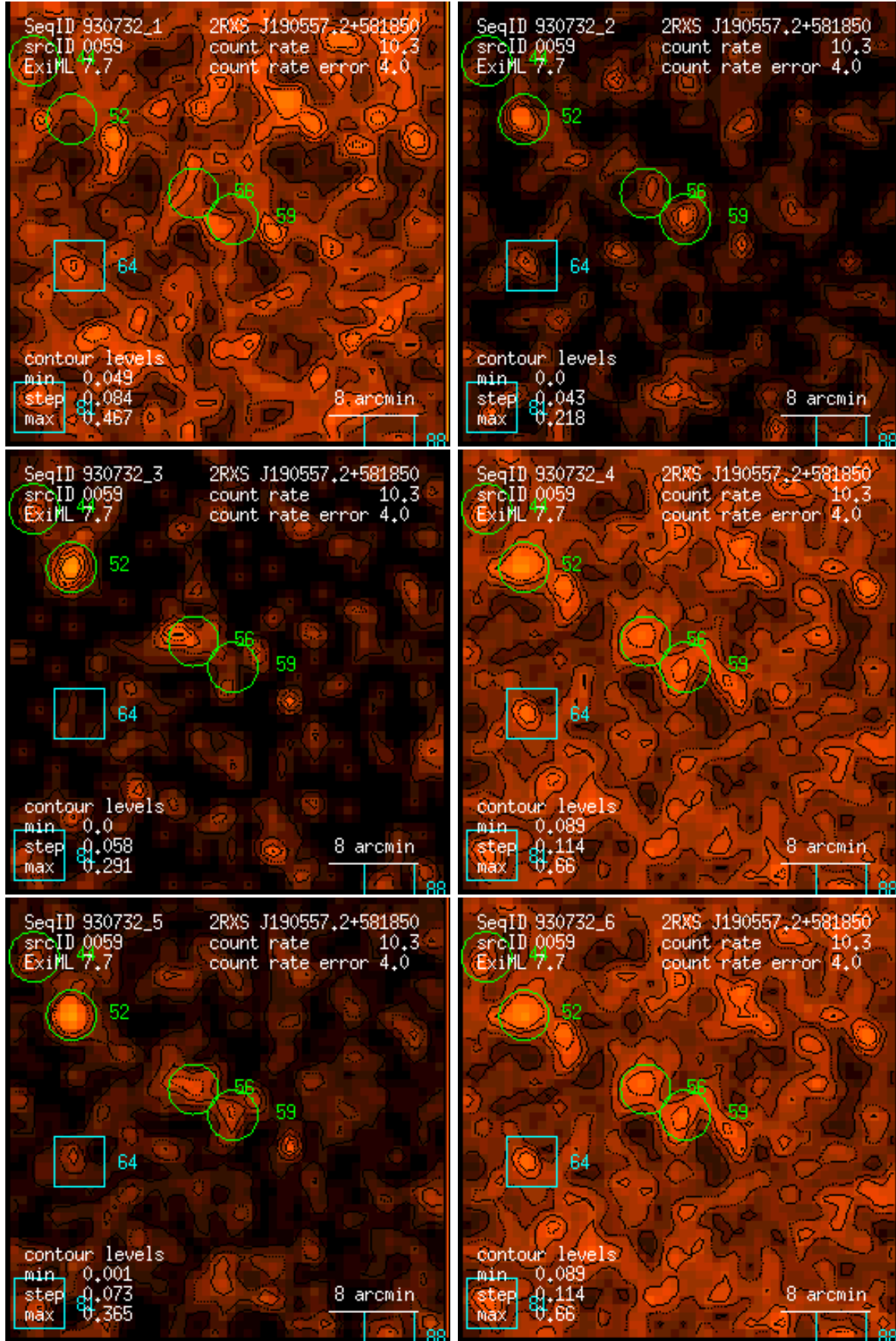
Figure 59: RASS 930732: detection 0059: band rate images, Gaussian filter: (1) PSPC channels 11 – 41, (2) 52 – 90, (3) 91 – 201, (4) 11 – 235, (5) 52 – 201, (6) 11 – 201. Broad band rates in counts/ks. Band rate contour levels in counts/ks/arcmin 2 .
