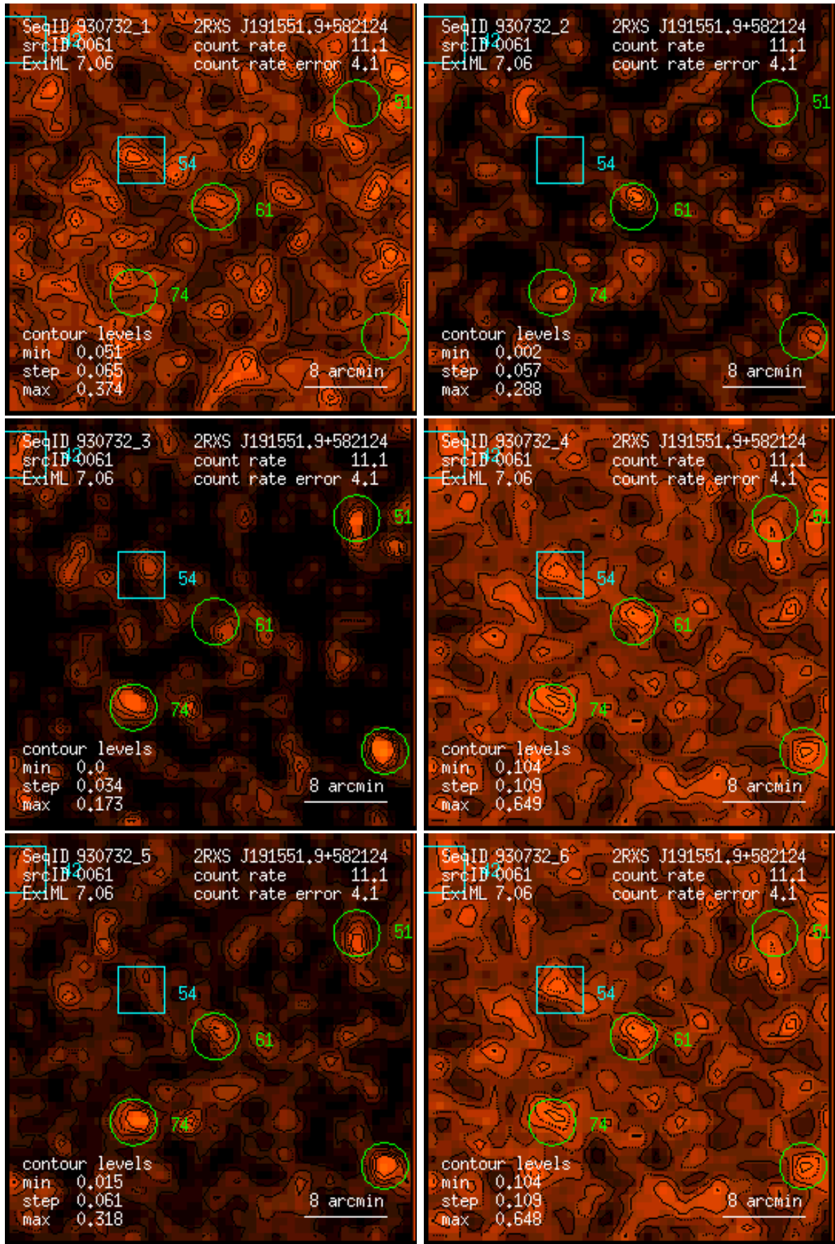
Figure 61: RASS 930732: detection 0061: band rate images, Gaussian filter: (1) PSPC channels 11 – 41, (2) 52 – 90, (3) 91 – 201, (4) 11 – 235, (5) 52 – 201, (6) 11 – 201. Broad band rates in counts/ks. Band rate contour levels in counts/ks/arcmin 2 .
