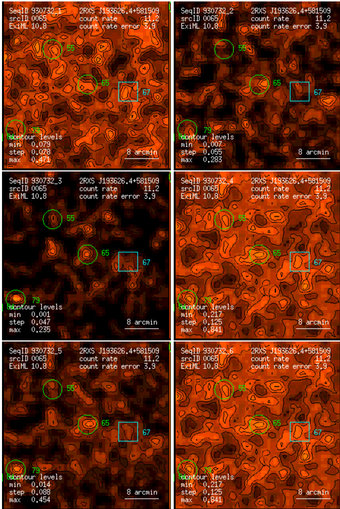
Figure 65: RASS 930732: detection 0065: band rate images, Gaussian filter: (1) PSPC channels 11 – 41, (2) 52 – 90, (3) 91 – 201, (4) 11 – 235, (5) 52 – 201, (6) 11 – 201. Broad band rates in counts/ks. Band rate contour levels in counts/ks/arcmin 2 .
