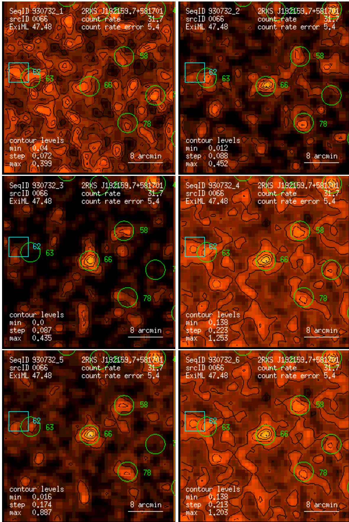
Figure 66: RASS 930732: detection 0066: band rate images, Gaussian filter: (1) PSPC channels 11 – 41, (2) 52 – 90, (3) 91 – 201, (4) 11 – 235, (5) 52 – 201, (6) 11 – 201. Broad band rates in counts/ks. Band rate contour levels in counts/ks/arcmin 2 .
