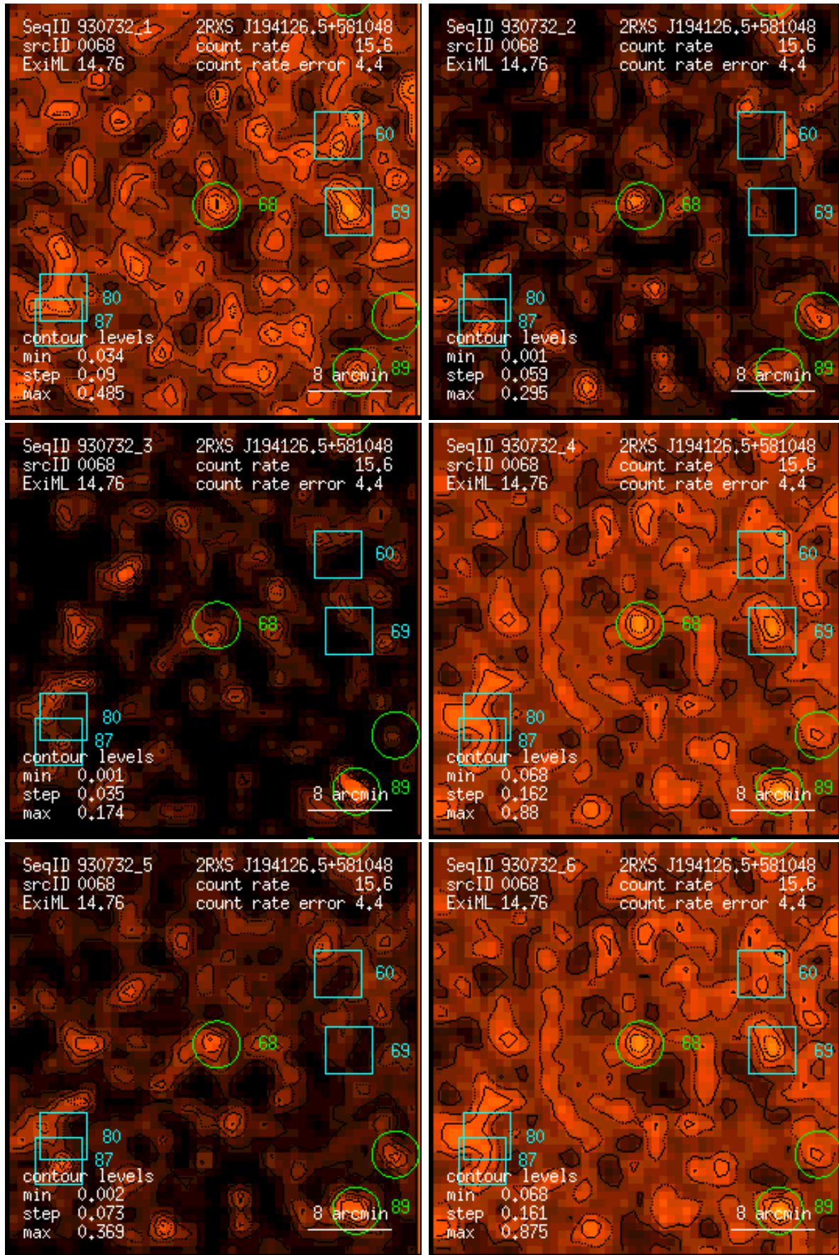
Figure 68: RASS 930732: detection 0068: band rate images, Gaussian filter: (1) PSPC channels 11 – 41, (2) 52 – 90, (3) 91 – 201, (4) 11 – 235, (5) 52 – 201, (6) 11 – 201. Broad band rates in counts/ks. Band rate contour levels in counts/ks/arcmin 2 .
