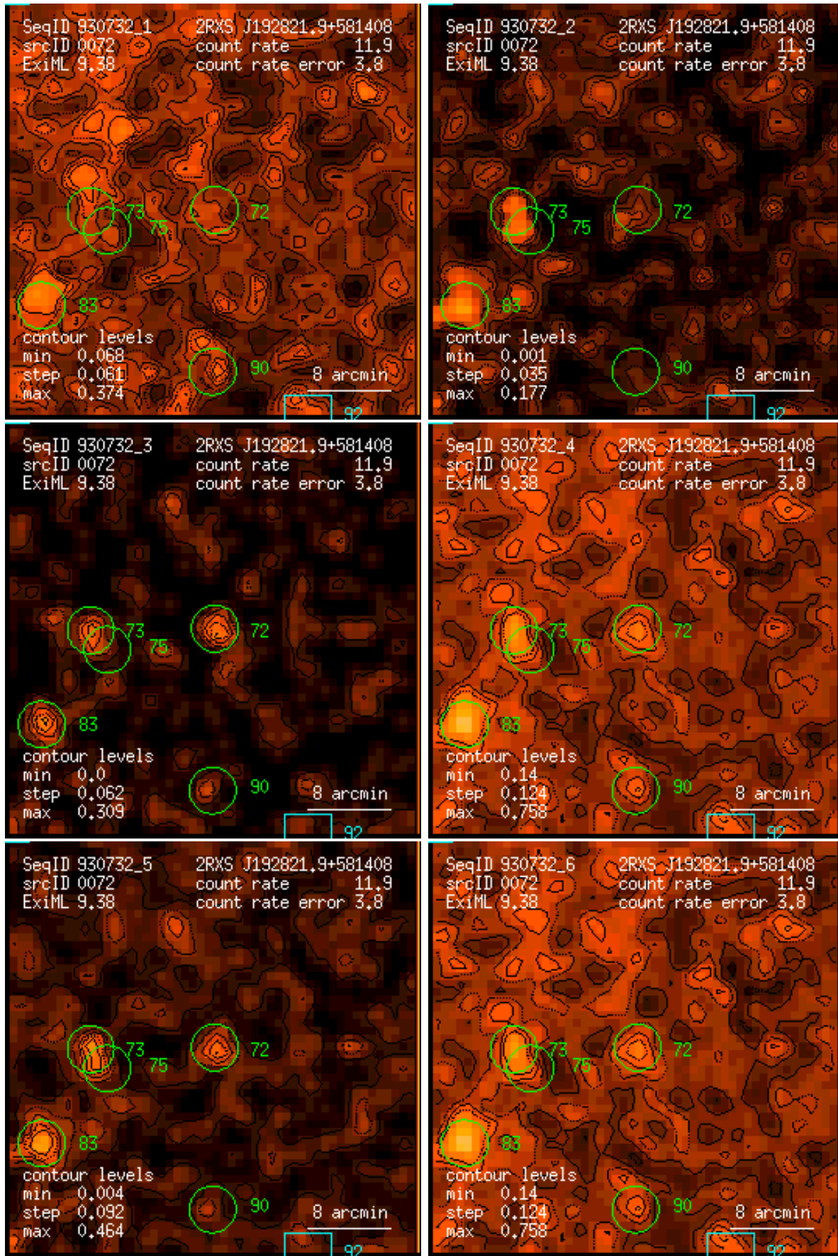
Figure 72: RASS 930732: detection 0072: band rate images, Gaussian filter: (1) PSPC channels 11 – 41, (2) 52 – 90, (3) 91 – 201, (4) 11 – 235, (5) 52 – 201, (6) 11 – 201. Broad band rates in counts/ks. Band rate contour levels in counts/ks/arcmin 2 .
