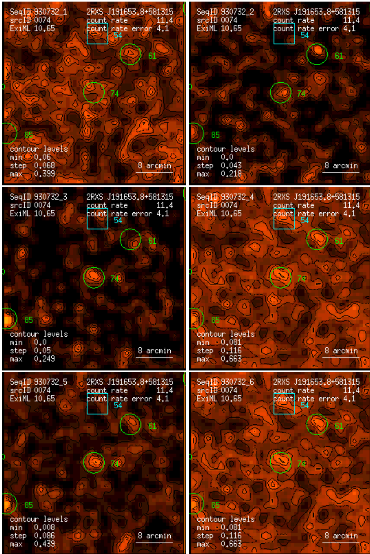
Figure 74: RASS 930732: detection 0074: band rate images, Gaussian filter: (1) PSPC channels 11 – 41, (2) 52 – 90, (3) 91 – 201, (4) 11 – 235, (5) 52 – 201, (6) 11 – 201. Broad band rates in counts/ks. Band rate contour levels in counts/ks/arcmin 2 .
