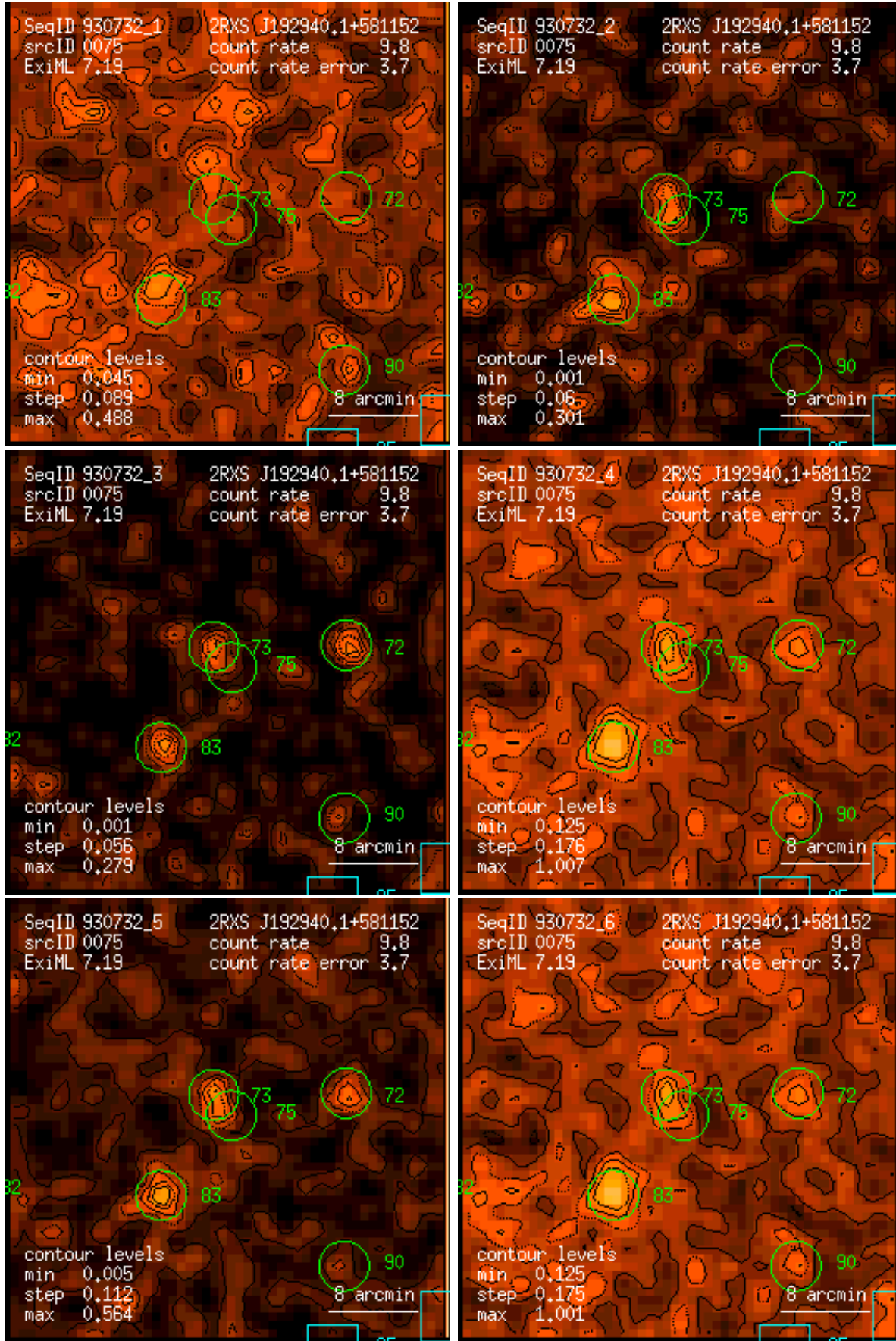
Figure 75: RASS 930732: detection 0075: band rate images, Gaussian filter: (1) PSPC channels 11 – 41, (2) 52 – 90, (3) 91 – 201, (4) 11 – 235, (5) 52 – 201, (6) 11 – 201. Broad band rates in counts/ks. Band rate contour levels in counts/ks/arcmin 2 .
