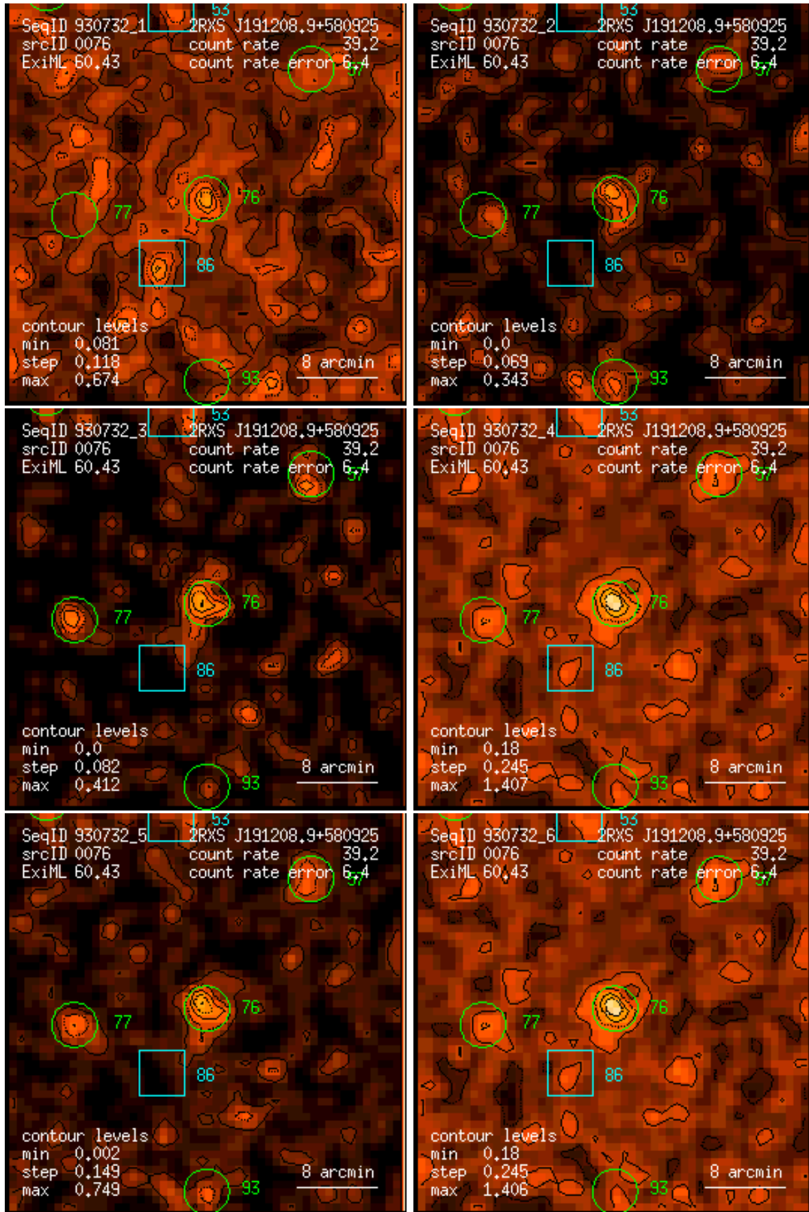
Figure 76: RASS 930732: detection 0076: band rate images, Gaussian filter: (1) PSPC channels 11 – 41, (2) 52 – 90, (3) 91 – 201, (4) 11 – 235, (5) 52 – 201, (6) 11 – 201. Broad band rates in counts/ks. Band rate contour levels in counts/ks/arcmin 2 .
