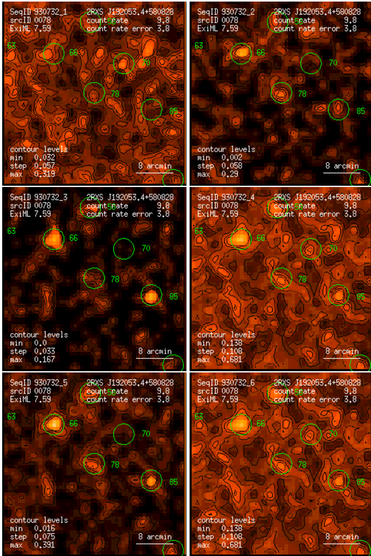
Figure 78: RASS 930732: detection 0078: band rate images, Gaussian filter: (1) PSPC channels 11 – 41, (2) 52 – 90, (3) 91 – 201, (4) 11 – 235, (5) 52 – 201, (6) 11 – 201. Broad band rates in counts/ks. Band rate contour levels in counts/ks/arcmin 2 .
